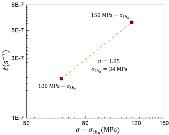
(e) \dot{\epsilon} vs (\sigma - \sigma_{th0}) for AA2219-T4
