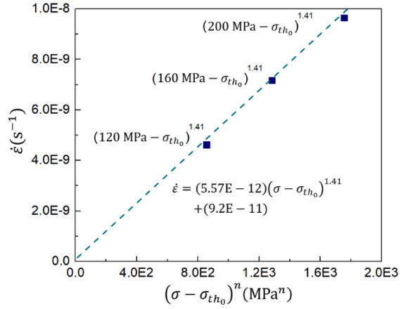
(b) \dot{\epsilon} vs (\sigma - \sigma_{th0})^n for AA2195-T3
