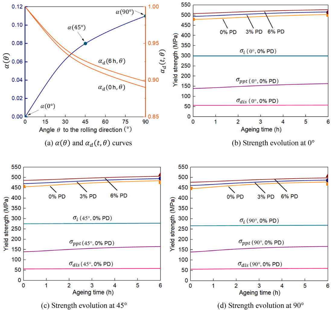
Fig. 10. The strength evolution prediction results. (a) presents the NURBS curve of \alpha(\theta) and the corresponding \alpha_d(t, \theta) at 0 and 6 h in creep-ageing. The solid symbols in (a) are the values of \alpha(\theta) for establishing the curve. (b) to (d) demonstrate respectively the strength evolution prediction results at 0°, 45°, and 90° for 0%, 3%, 6% pre-deformation (PD) extents. The solid symbols in (b) to (d) denote experimental data from (Wang et al., 2023c).
