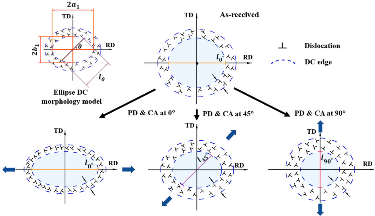
Fig. 2. Schematic of ellipse dislocation cell (DC) morphology and its evolution with PD and creep-ageing at the same directions along 0°, 45°, and 90° to the rolling direction. PD & CA refers to pre-deformation and creep-ageing. l_\theta denotes the DC length at angle \theta to the rolling direction.
