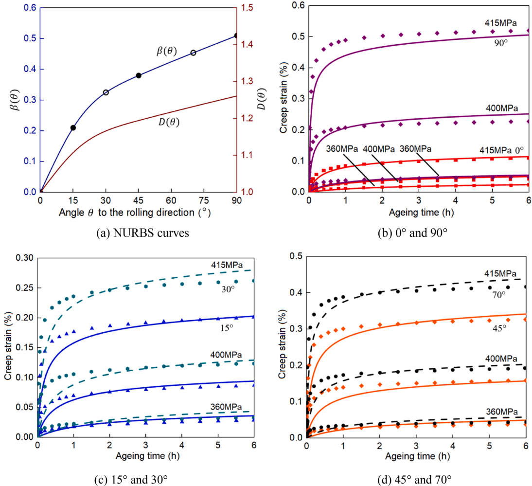
Fig. 6. Comparison of prediction results and experimental data for the 3rd generation Al-Li alloy when creep-aged at different directions and stresses at 143^\circ\text{C} . (a) displays the NURBS curve of \beta(\theta) and D(\theta) . (b) to (d) compare the prediction results (lines) with experimental ones (symbols) from (Wang et al., 2023b). The dashed lines of 30^\circ and 70^\circ represent the prediction results obtained from the model calibrated without these data.
