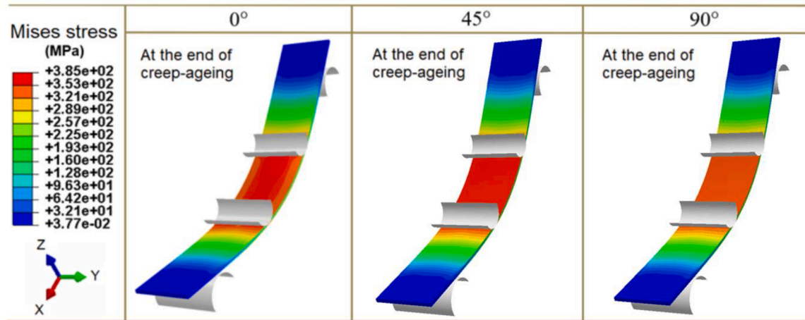
(a) Simulated stress distributions at the end of creep-ageing at 0^\circ , 45^\circ , and 90^\circ
