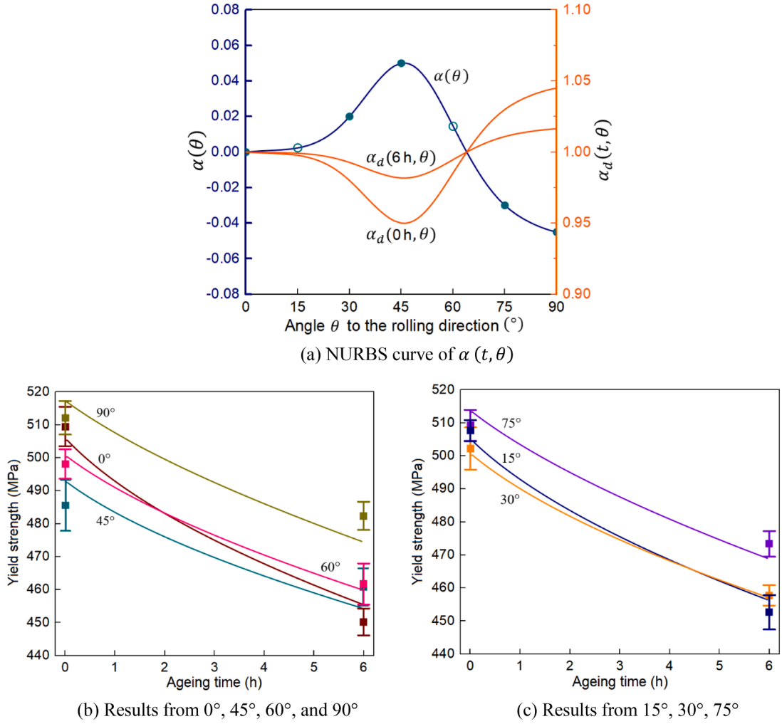
Fig. 12. The NURBS curve of \alpha(\theta) and strength evolution prediction results. The solid symbols in (a) are used for establishing the curve, the hollow circles are prediction values obtained from the established curve. (b) and (c) present the strength evolution prediction results at different angles ranging from 0^\circ to 90^\circ . The solid symbols with error bars in (b) and (c) stand for the experimental data from (Chen et al., 2022).
