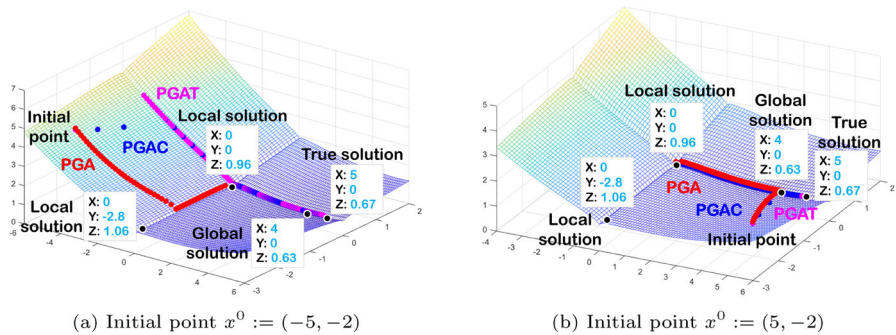
Fig. 1 Consider problem (1) and the regularization problem (2) with A := \begin{bmatrix} -0.2554 & 0.0778 \\ 0.1084 & -0.1811 \end{bmatrix} , b := \begin{bmatrix} -1.2770 \\ 0.5420 \end{bmatrix} , \varepsilon = 0 , \varphi(x) = \ell_{1/2} penalty and \lambda := 0.3 . If starting from (-5, -2) , the PGA only converges to a local solution (0, 0) , and the PGAC and PGAT first go to the neighborhood of the local solution (0, 0) , are then able to escape from this local solution, and finally converge to an approximation of the true sparse solution (5, 0) , see (a). If starting from (5, -2) , PGA and PGAC will have the same behaviour as starting from (-5, -2) . However PGAT will directly converge to an approximation of the true sparse solution (5, 0) , see (b). Note that this true sparse solution is also an approximate global solution of the \ell_{1/2} regularization problem
