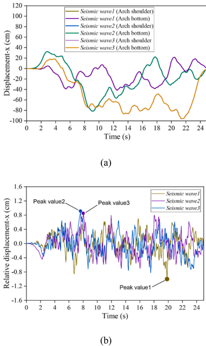
Fig. 14. (a) Displacement time-history curves; (b) Relative-dis time-history curves of the segmental linings (Yang et al., 2022b).
