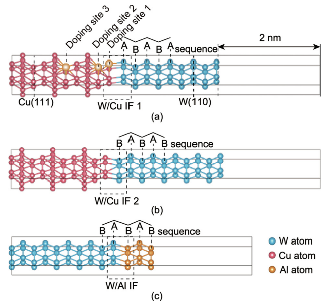
Fig. 9. Atomic models of different interfaces. (a) W/Cu IF 1, where different substitution sites of Al in a Cu lattice are indicated; (b) W/Cu IF 2; (c) coherent W/bcc Al. IF stands for interface.
