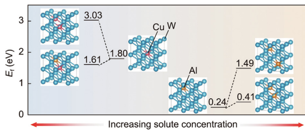
Fig. 8. Calculated formation energies ( E_f ) of dissolving Cu and Al into W at different concentrations and atomic configurations.
