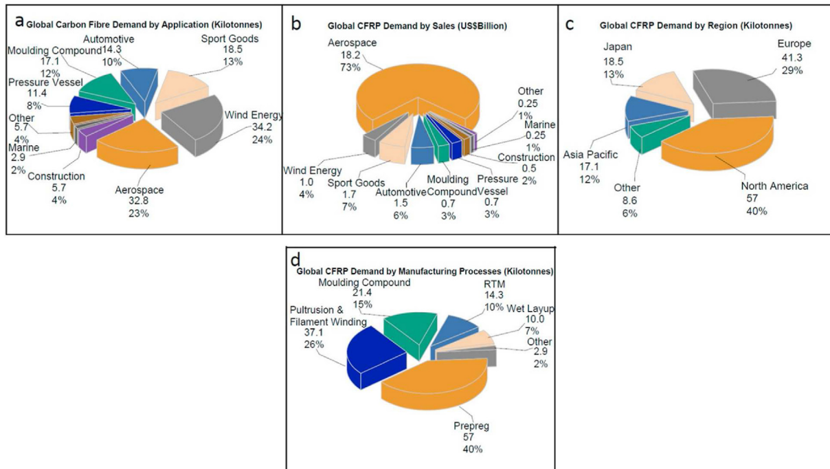
Fig. 10 – Worldwide CFRPC requirement in the year 2018 segmented by (a) Application in different sectors by quantity and percentage, (b) Trades, (c) Region, (d) Production method [72,76–78].
