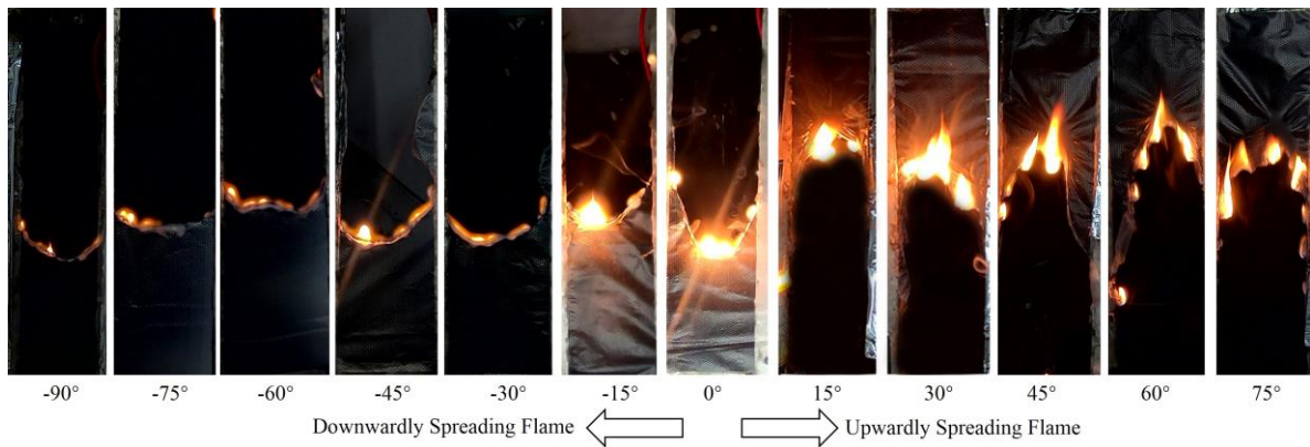
Fig. 6. Flame appearance under different angles ( \tau = 20 \mu\text{m} ).
