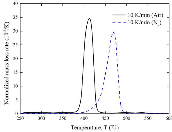
Fig. A1. DTG curves of HDPE at the heating rate of 10 K/min.
