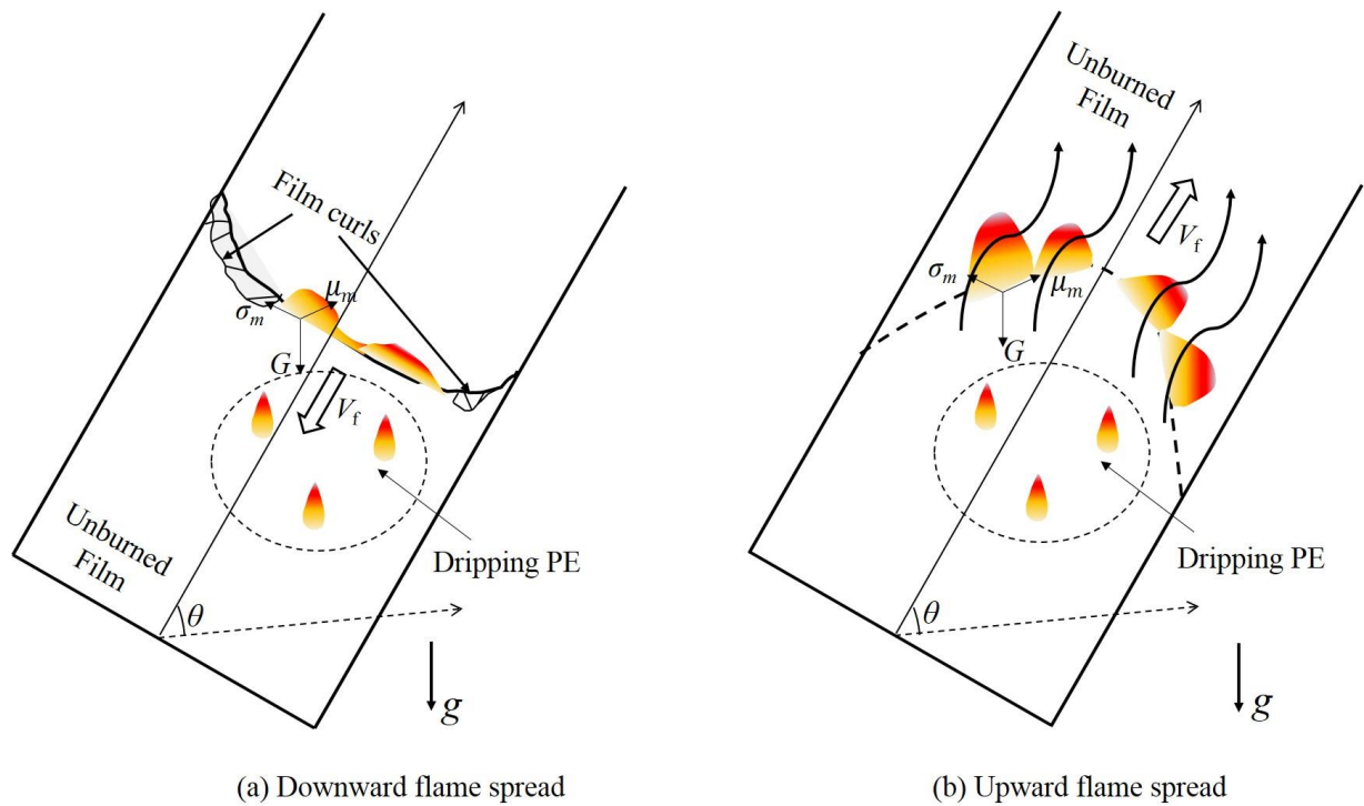
Fig. 10. Schematic diagram of the flame spread over PE film with different fuel inclinations, (a) downward flame spread and (b) upward flame spread.
