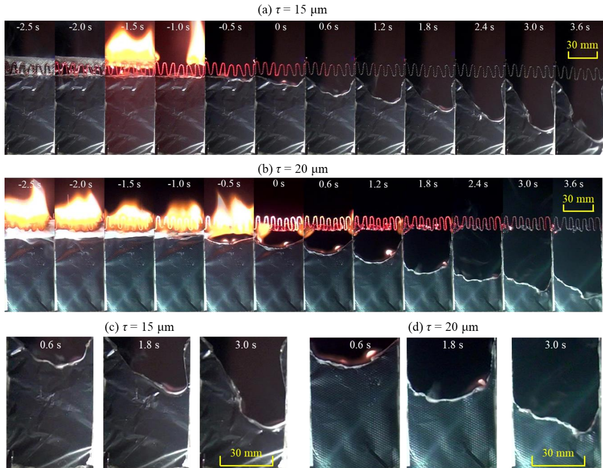
Fig. 3. Images of the flame spread process under microgravity environment, (a) 15- \mu\text{m} PE film, and (b) 20- \mu\text{m} PE film (also see Videos S1 and S2).
