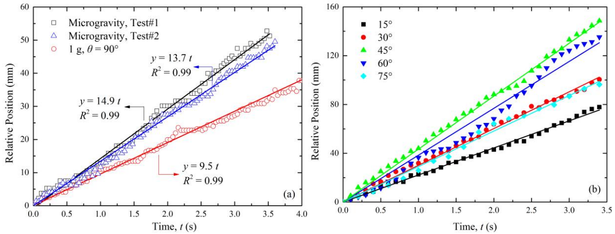
Fig. A2. The time evolution of the flame leading edge position for the film with a thickness of 20 \mu\text{m} for (a) downward flame spread and microgravity flame spread (b) upward flame spread.
