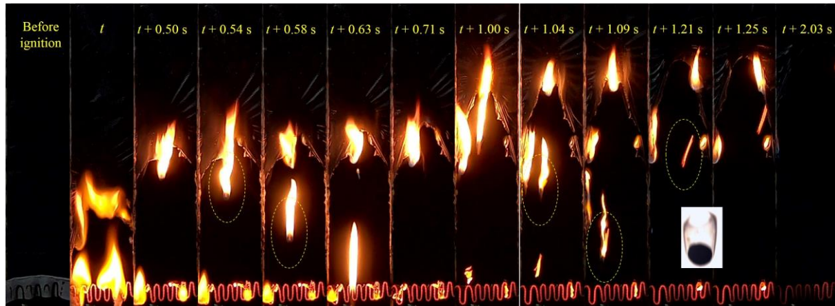
Fig. 9. A typical dripping and extinction process of upward flame spread ( \theta = 90^\circ ) with the 20- \mu\text{m} thin PE film (see Video S5).
