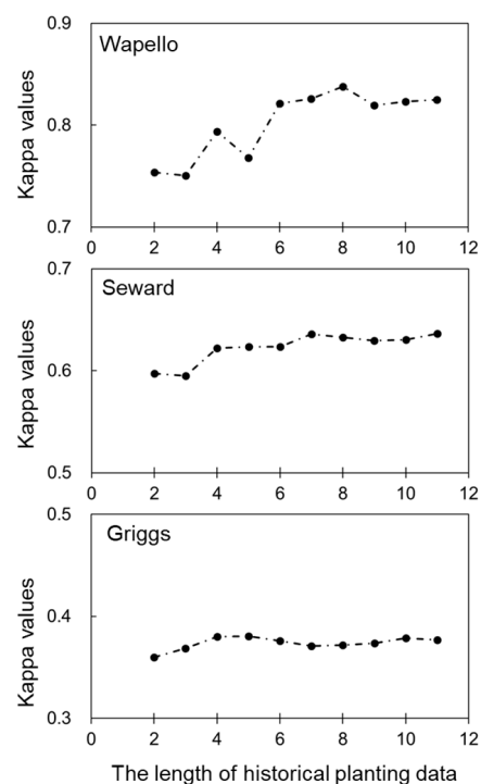
Figure 9. The performance of CDL-based crop classification (Kappa values) using different numbers of years of historical planting data at the three U.S. sites.
