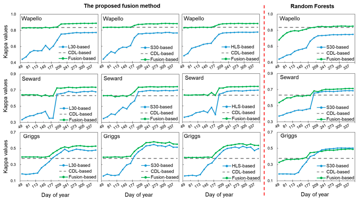
Figure 3. The performance of crop classification using the proposed fusion method (left) and the random forest model (right) at the three U.S. sites. In each panel, we show the kappa values for the CDL-based, spectral-based (L30, S30, or HLS), and the fusion-based crop classifications as the growing season progresses.
