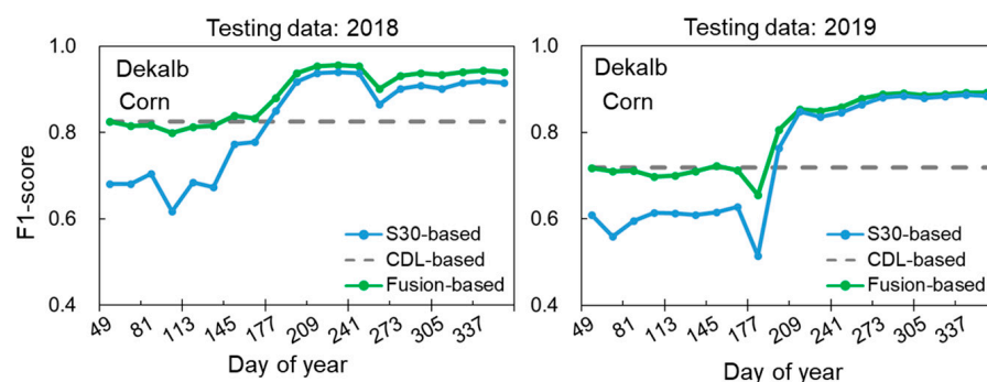
Figure 13. The performance of CDL-based, S30-based, and fusion-based classifications for corn in the Dekalb County (located in Illinois) using the years 2018 and 2019 as the testing data.
