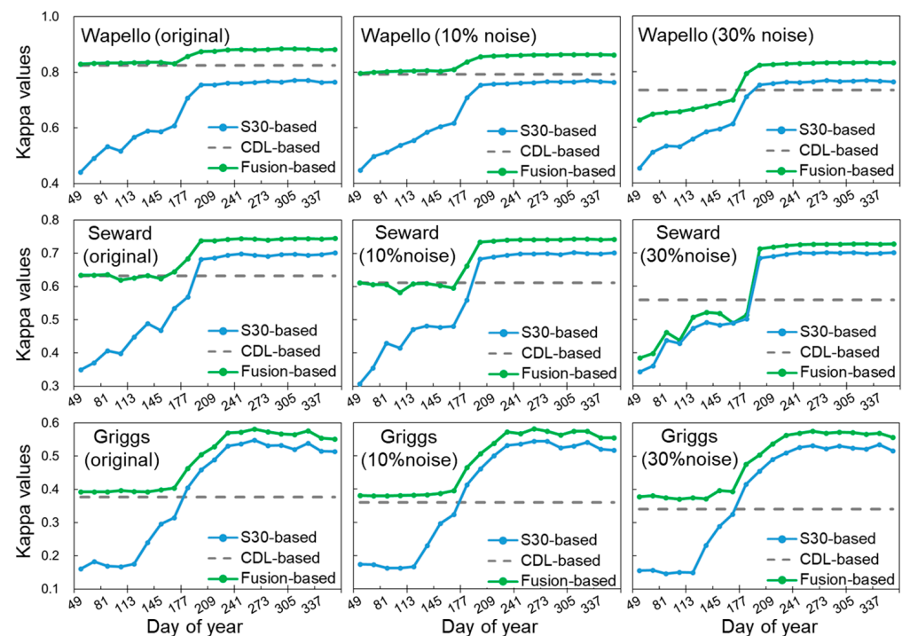
Figure 11. The performance of crop classification through the crop season under different scenarios with simulated different levels of error (10% and 30%) in the historical CDL datasets.
