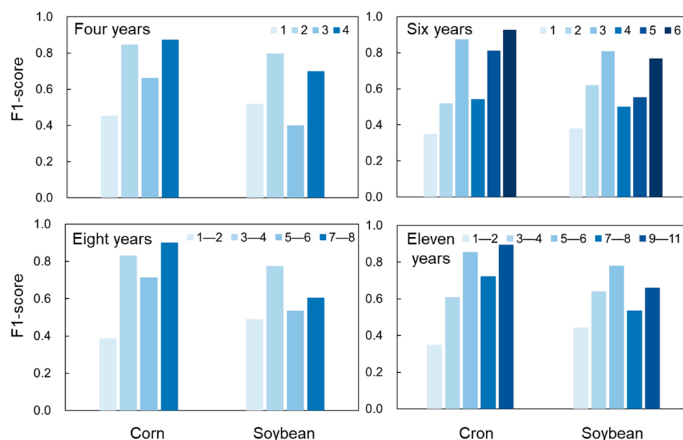
Figure 10. The relationship between crop planting frequency and crop classification performance. Here, crop planting frequency is calculated as the number of times (e.g., 1–4 in the first panel) corn (or soybean) were planted in the past (e.g., four years in the first panel).
