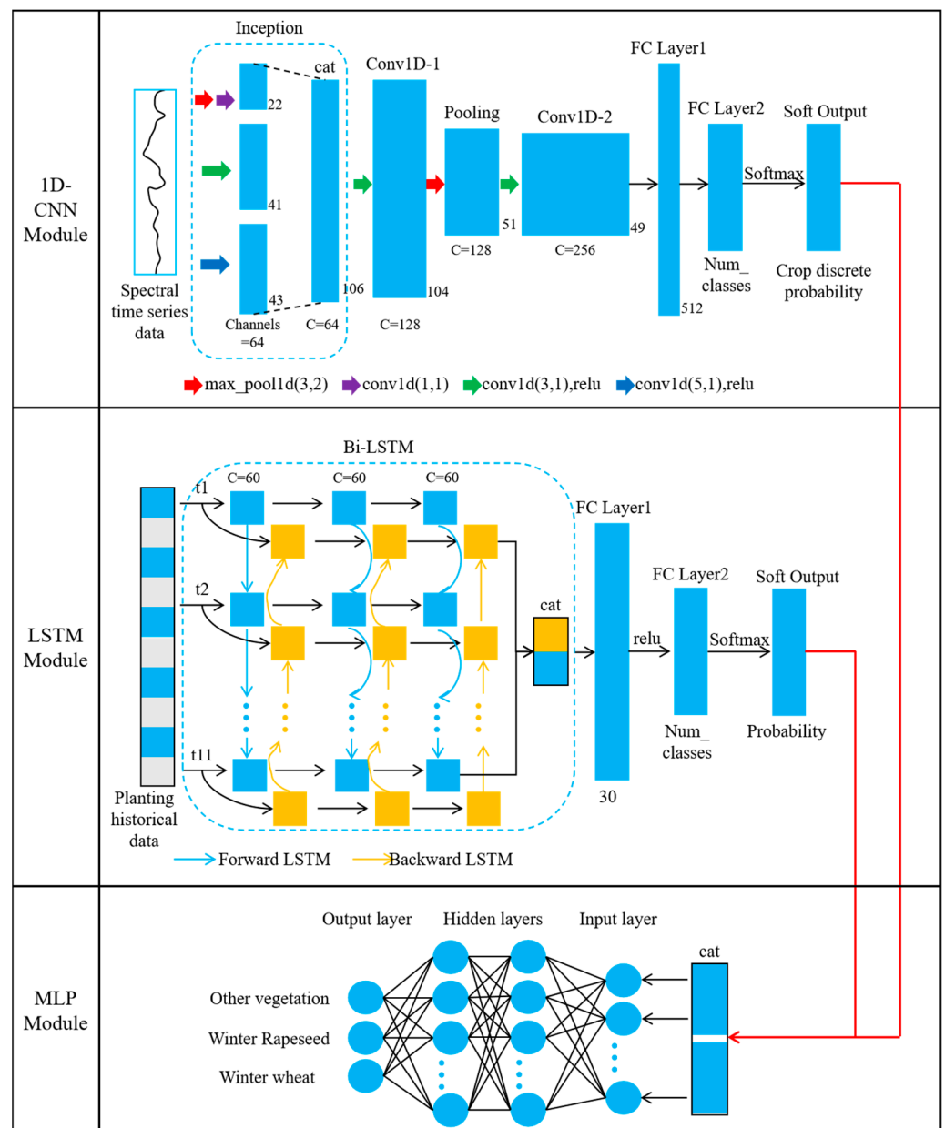
Figure 1. The neural network structure of the proposed within-season crop identification model.
