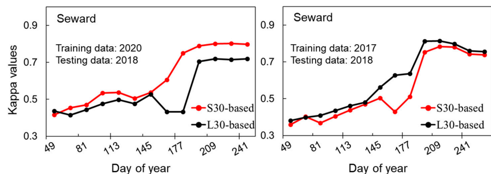
Figure 5. The performance of spectral-based (L30 or S30) crop classification at the Seward site using the data from different years as the training data.
