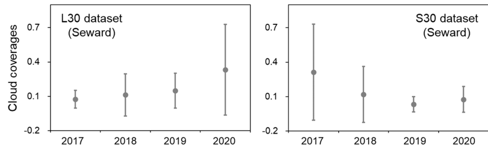
Figure 4. The cloud coverage (mean and standard deviation) in the L30 and S30 images acquired during the period (145–193 DOY) at the Seward site in each year.
