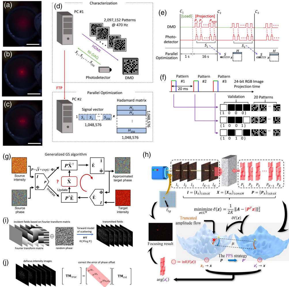
Fig. 3 Representative TM methods with high performance. Demonstration of analytical real-part TM-based method. 21 (a) speckles before optimization; (b) single focus after optimization; (c) three foci after optimization; (d) PC#1 is used to synchronize a DMD and a photodetector for pattern display and measurement and PC#2 is for the parallel optimization; (e) the data flow diagram; (f) DMD displaying workflow with a custom HDMI protocol, where the first four patterns are for error correction and the next 20 patterns are for probing patterns. (g) The flowchart of the GGS algorithm to retrieve the unknown TM. 25 (h) A method of PPS-AF, 59 using the PPS strategy to smooth the high-dimensional hyperplane (with many local minimums) to achieve fast convergence toward the global optimum. TM retrieval with fast Fourier transform (FFT): (i) encoding the Fourier transform matrix into the input wavefront allows FFT to accomplish the inverse algorithm of TM; and (j) phase error of TM can be corrected by the defocus images. 60 Images (a)–(f), (g), (h), and (i), (j) are reproduced with permission from Refs. 21, 25, 59, and 60, respectively.
