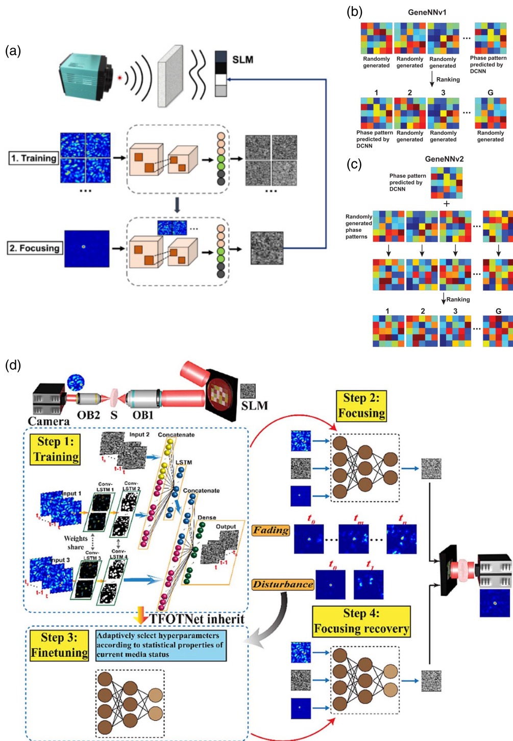
Fig. 5 Representative learning-based precompensation WFS. A hybrid realization by reinforcing GA with DNN prediction: 74 (a) the workflow, train the network first to output phase patterns, which will be combined with the phase patterns generated by GA; two different combinations (i.e., GeneNNv1 and GeneNNv2) between GA and DNN in (b) and (c). (d) Smart focusing through a moving diffuser with TFOTNet: 75 the network is first trained for initial focusing and then fine-tuned by monitoring the time-varying focus/speckles for focusing recovery. Images (a)–(c) and (d) are reproduced with permission from Refs. 74 and 75, respectively.
