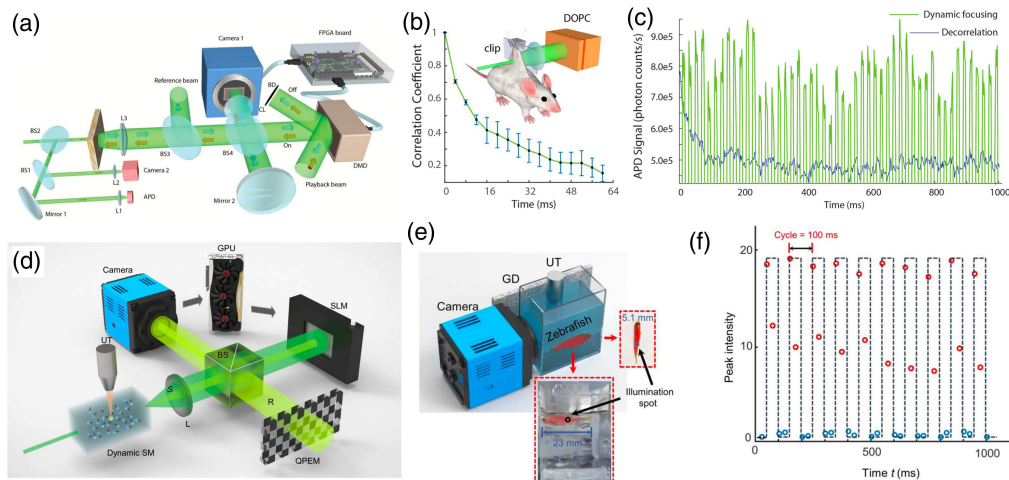
Fig. 6 Representative fast DOPC dynamic focusing on millisecond scale. Dynamic focusing with a FPGA-DMD configuration in a DOPC system: 40 (a) the schematic experimental setup; (b) decorrelation of the back on a living mouse; and (c) dynamic focusing during the decorrelation. High-speed single-shot TRUE focusing with full phase modulation: 77 (d) DOPC setup with a QPEM and a GPU; (e) configuration for TRUE focusing in between the zebrafish and a ground glass diffuser; and (f) dynamic focusing realized in (e). Images (a)–(c) and (e), (f) are reproduced with permission from Refs. 40 and 77, respectively.
