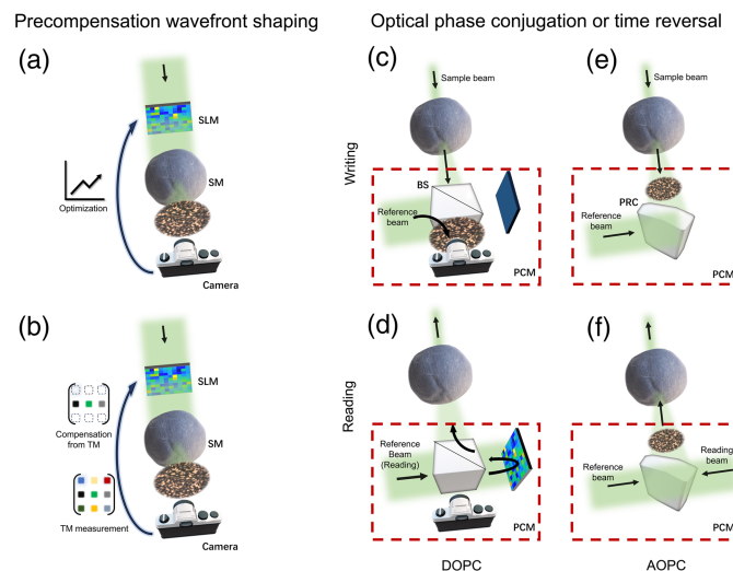
Fig. 1 Illustration of the two types of WFS implementations. Precompensation WFS: (a) online iterative optimization and (b) TM-based method. (c)–(f) OPC or optical time reversal: (c), (d) DOPC; (e), (f) AOPC; (c), (e) hologram writing; and (d), (f) hologram reading. Abbreviations: SLM, spatial light modulator; SM, scattering medium; TM, transmission matrix; PCM, phase conjugation mirror; PRC, photorefractive crystal; OPC, optical phase conjugation; AOPC and DOPC: analogue OPC and digital OPC.
