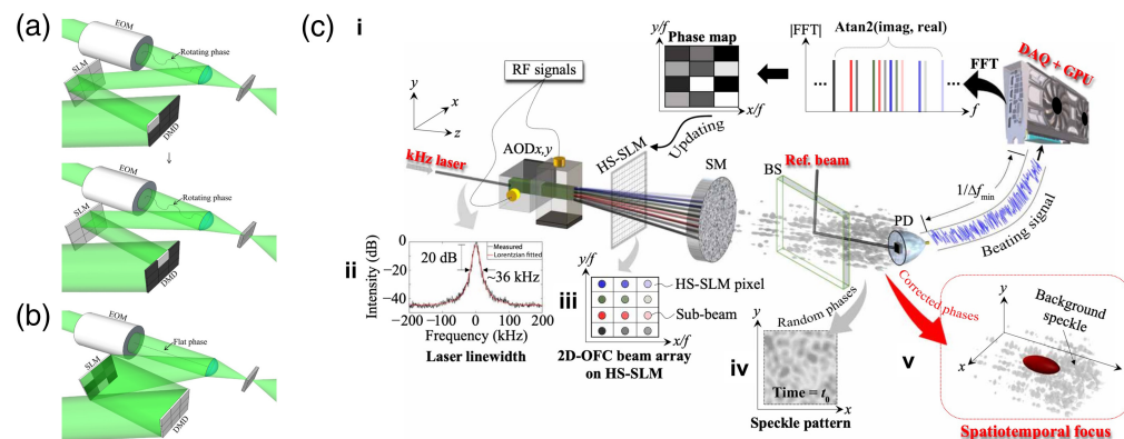
Fig. 2 Representative realizations of employing more than one SLM for enhanced performance. Combination between a phase-only SLM and a DMD: (a) the phase measurement process, in which a flat phase is displayed on the SLM, and light reflected from each DMD superpixel illuminates a corresponding SLM superpixel while the EOM provides the phase modulation; and then (b) all DMD pixels are set to be on and optimized phase is displayed on the SLM, while the EOM remains a flat phase. (c) Hybrid modulation with an optical frequency comb, AOD, and an NLC-SLM. The HS-SLM (high-speed SLM) in (c) is a NLC-SLM. Images (a) and (b) are reproduced with permission from Ref. 54 and image (c) is reproduced with permission from Ref. 44.
