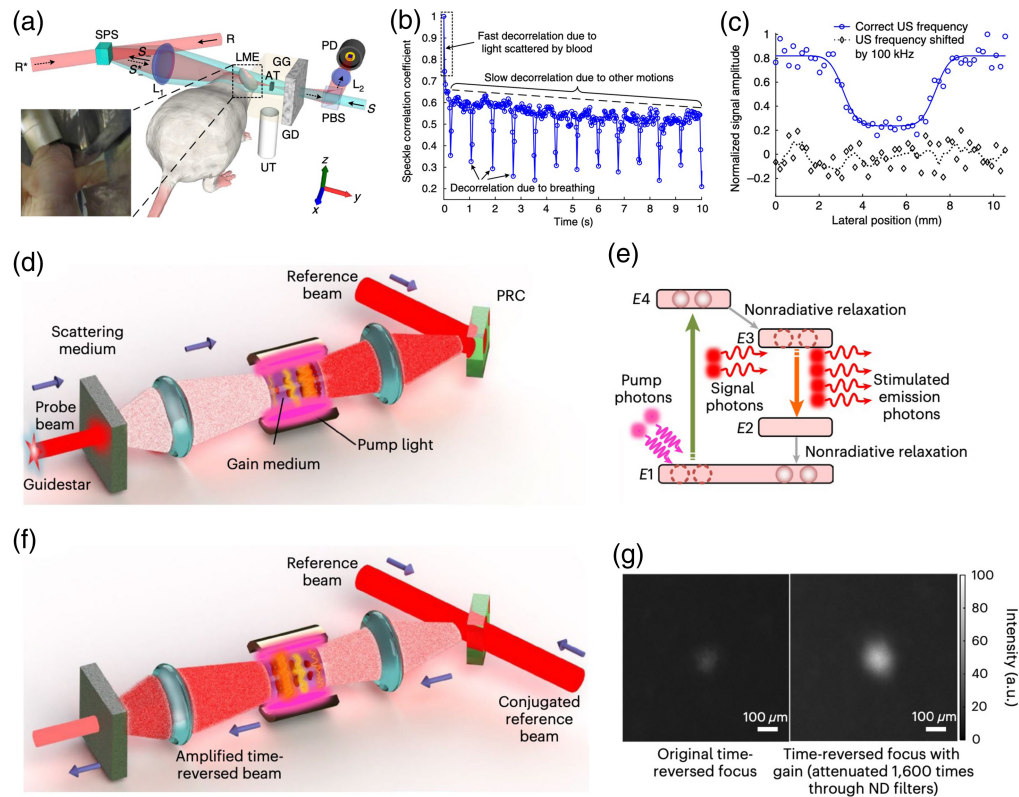
Fig. 7 Representative realizations of efficient AOPC. Focusing inside dynamic scattering medium with near-infrared TRUE light in AOPC: (a) experimental schematic to focused diffused light and image an absorptive target between a diffuser and a living mouse; (b) decorrelation of speckles from a living mouse; and (c) one-dimension profile image of the absorptive target. High-speed and high-gain AOPC: (d) the recording process and (f) the reading process of the AOPC system; (e) diagram of the four-level gain medium of stimulated emission light amplification; and (g) focusing with and without the energy gain. Images (a)–(c), (d)–(g) are reproduced with permission from Refs. 27 and 87, respectively.
