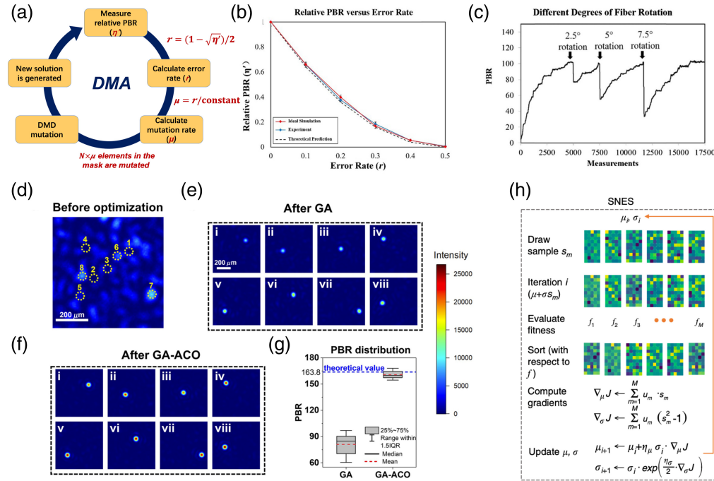
Fig. 4 Representative adaptive and efficient precompensation algorithms. The dynamic mutation algorithm (DMA): 29 (a) the flowchart of DMA; (b) the modulation square law validated by simulation and experiment; and (c) the recovery of PRB by DMA under multiple rotations applied to the MMF. GA-ACO algorithm: 30 (d) speckles before optimization; (e), (f) focusing optimization with GA and GA-ACO, respectively; and (g) the statistics comparison for PBR between the GA and GA-ACO. (h) Flowchart of SNES algorithm. 71 Images (a)–(c), (d)–(g), and (h) are reproduced with permission from Refs. 29, 30, and 68, respectively.
