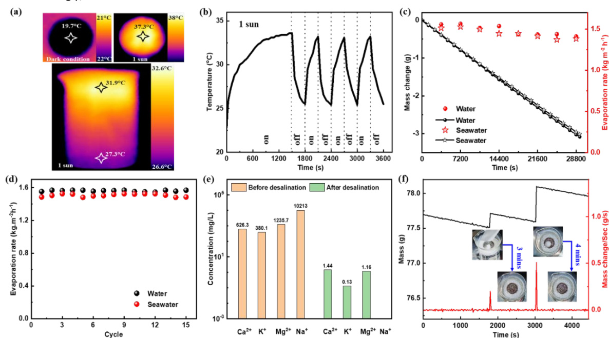
Fig. 7 (a) Thermal images of OPU under dark condition, 1 sun and temperature distribution of water at the top and the bottom of the beaker. (b) light on-off cycle test of OPU under 1 sun with 5-minute interval. (c) The 8 hours of long evaporation performance for tap water and natural seawater. (d) Cycle tests of evaporating water and seawater under 1 sun for 15 consecutive days. (e) ICP-OES result of concentration of \text{Ca}^{2+} , \text{K}^+ , \text{Mg}^{2+} and \text{Na}^+ before and after seawater desalination. (f) Salt rejection performance of the OPU.
