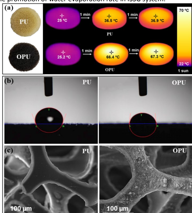
Fig. 5 Dry PU and OPU substrates: (a) thermal images before or after irradiation under 1 sun (b), WCA photos, (c) SEM images.
