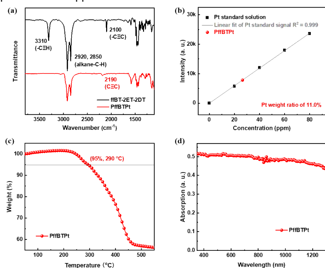
Fig. 2 (a) FTIR spectra of fFBT-2ET-2DT and PffBTPT. (b) ICP-OES curves of the PffBTPT. (c) TGA and (d) DRS curves of PffBTPT.
