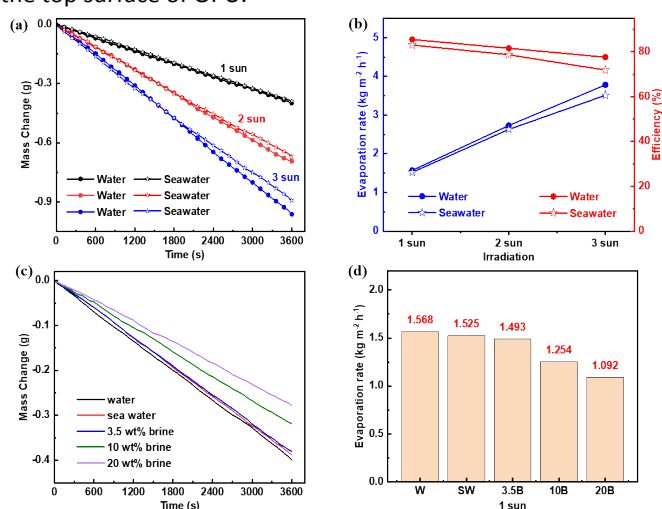
Fig. 6 (a) Mass change of water and seawater under 1 sun, 2 sun and 3 sun. (b) The corresponding evaporation rate and efficiency. (c) Mass change and (d) evaporation rate of water, seawater and brine waters under 1 sun.
