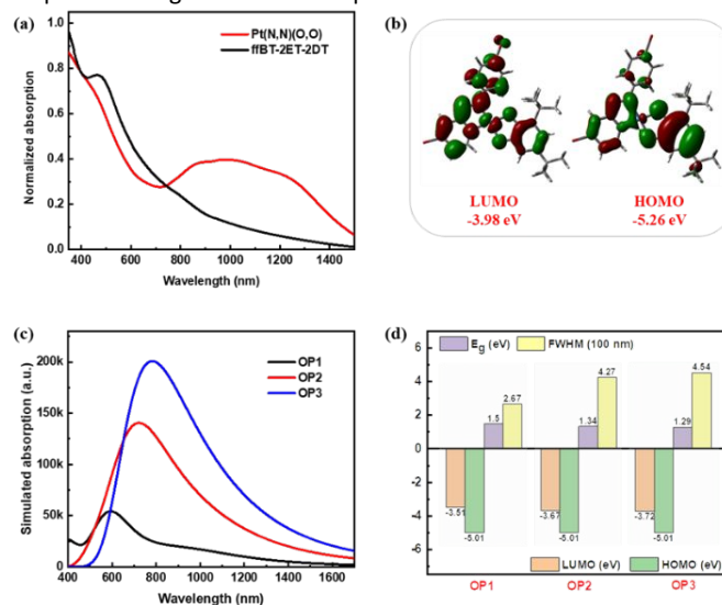
Fig. 3 (a) Absorption spectra of Pt(N,N)(O,O) and fFBT-2ET-2DT films. (b) Optimized S 0 geometry of Pt(N,N)(O,O) and the calculated LUMO and HOMO energy levels. (c) Simulated absorption spectra of OP1, OP2 and OP3. (d) Calculated LUMO, HOMO, E g and FWHM values.
