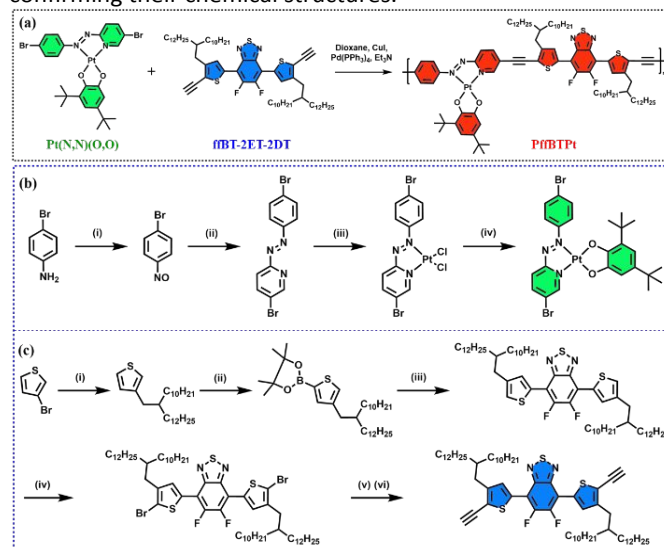
Fig. 1 The synthetic routes: (a) Polymer PffBTPT. (b) Complex monomer Pt(N,N)(O,O): (i) DCM, aq. 2KHSO 5 ·KHSO 4 ·K 2 SO 4 , rt. (ii) pyrrole, 2-amino-5-bromopyridine, aq. NaOH, 90 °C. (iii) acetonitrile: H 2 O (9:1), K 2 PtCl 4 , 100 °C. (iv) DCE, 3,5-di-tert-butylcatechol, Na 2 CO 3 , 80 °C. (c) Organic monomer ffBT-2ET-2DT: (i) THF, 11-(bromomethyl)tricosane, Mg, Ni(II)Cl 2 (dppp). (ii) THF, n -butyllithium, trimethyl borate, from -78 °C to rt. (iii) THF, 4,7-dibromo-5,6-difluoro-2,1,3-benzothiadiazole, Pd(PPh 3 ) 4 , Na 2 CO 3 , 60 °C. (iv) chloroform, N-bromosuccinimide, rt. (v) THF, trimethylsilylacetylene, CuI, Pd(PPh 3 ) 2 Cl, Et 3 N, rt. (vi) THF, tetra- n -butylammonium fluoride.
