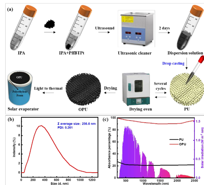
Fig. 4 (a) Preparation process of the used solar evaporator. (b) DLS curve of PffBTPT in PIA solution. (c) UV-Vis-NIR absorbance spectra of PU and OPU as well as solar radiation spectrum.
