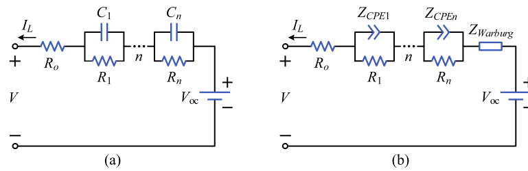
Fig. 17. Advanced equivalent circuit models of electric vehicle batteries. (a) Integral-order model. (b) Fractional-order model.
