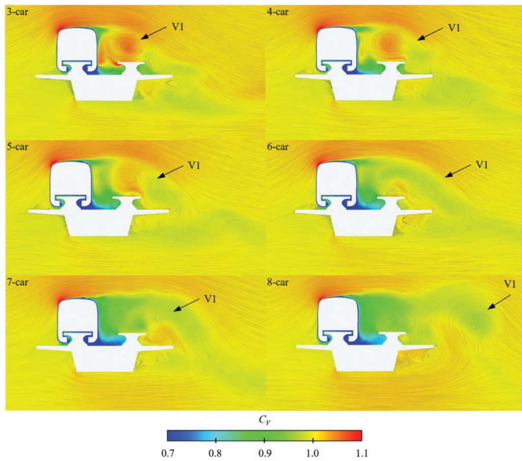
Figure 12: Velocity and flow structure distributions at cross-section X8 of different train lengths
