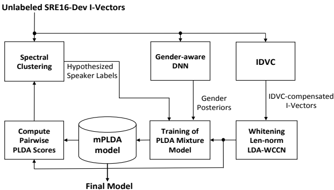
Fig. 1. Iterative retraining of the gender-aware PLDA mixture model
