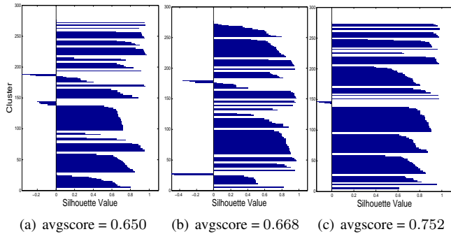
Fig. 2. Silhouette plots showing the quality of i-vector clusters produced by (a) Euclidean-AHC, (b) Cosine-AHC and (c) Iterative SC. Each silhouette pattern represents a cluster, and the silhouette values of individual samples are shown on the horizontal axis.
