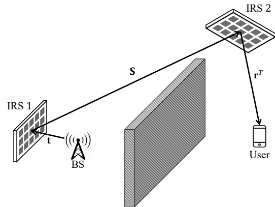
Fig. 1. A wireless communication system aided by two cooperative IRSs, where the user is served by the BS through the double reflection link (BS-IRS1-IRS2-user), while other links are unavailable due to severe blockage.
