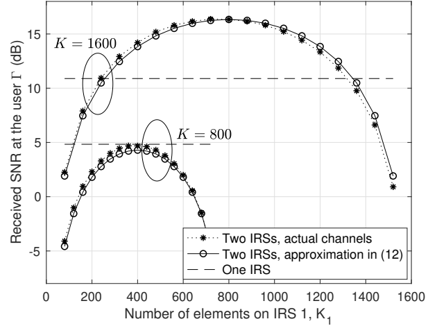
Fig. 4. Received SNR versus the number of elements on IRS 1, K_1 .
