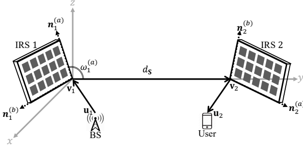
Fig. 3. Two IRSs in 3D space (the sizes of IRSs are exaggerated).
