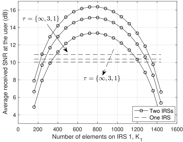
Fig. 5. Effect of Rician fading factor \tau on the performance.
