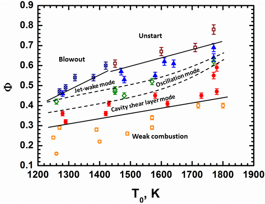
Figure 6. Regime nomogram of the flame stabilization modes
