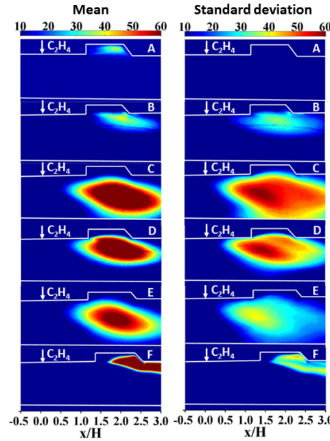
Figure 2. Mean and standard deviation images for \text{CH}^* chemiluminescence for Cases A-F
