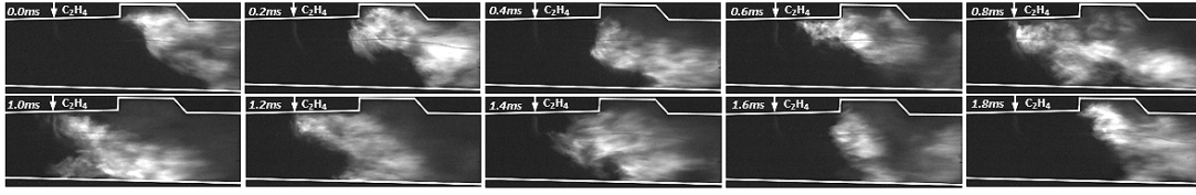
Figure 7 Time resolved CH* chemilluminescence images in Case D . Exposure time is 39 \mu s and sampling frequency 25000 fps.
