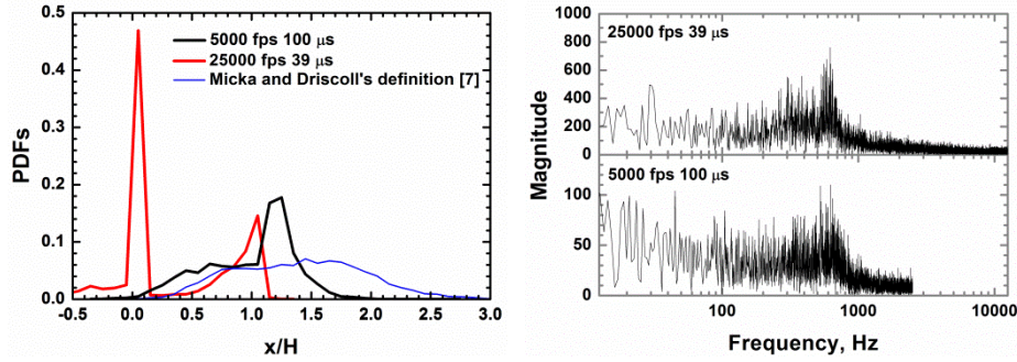
Figure 8 (a) PDFs of flame locations and (b) FFT of flame locations in Case D.
