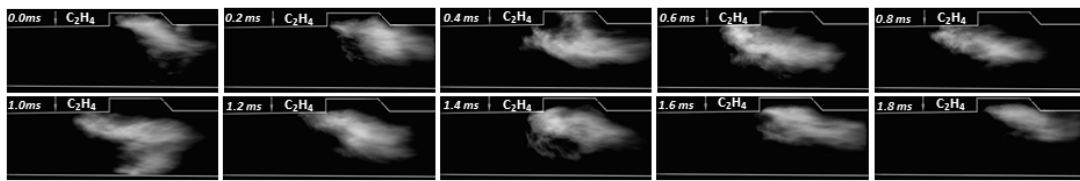
Figure 5. Time resolved \text{CH}^* chemiluminescence images in Case D . Exposure time is 100 \mu s and sampling frequency 5000 fps.
