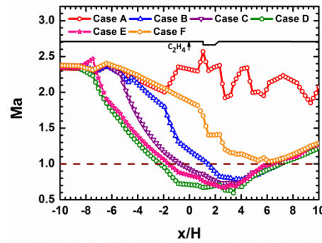
Figure 4. Calculated Mach number distributions for Cases A-F
