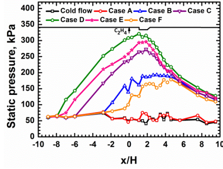
Figure 3. Measured wall static pressure profiles for Cases A-F
