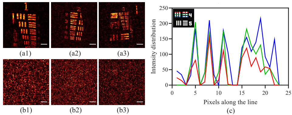
Fig. 3. Reconstruction results of a resolution target: (a1)–(a3) Group 1, Group 2 and Group 3 of the resolution target recovered by the proposed method respectively using 10 ml, 4 ml and 5 ml milk to be continuously dropped into water tank and a stirrer at 500 rpm. (b1)–(b3) Group 1, Group 2 and Group 3 of the resolution target recovered by using GI. (c) Intensity distributions of one-dimensional profiles in the recovered resolution target (i.e., element 4 of Group 3) using the proposed method. The inset on the top left corner of (c) is original image only for better visualization and marking. Scale bar: 1 mm.
