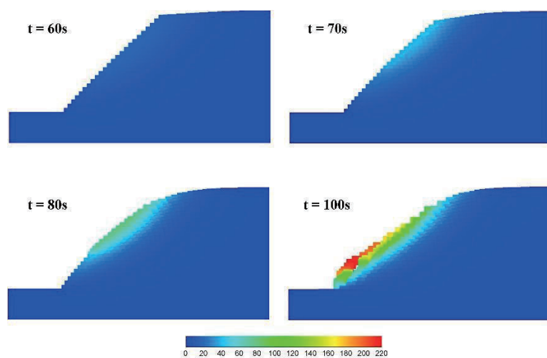
Fig. 3. Post-failure soil displacement (unit: mm) at four different times calculated using MPM.
