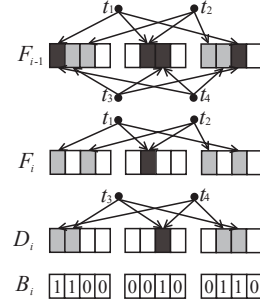
Fig. 2: An example of creating a Bloom filter of missing tags: F_{i-1} is the (i - 1) th physical-layer snapshot with four tags, where a white rectangle represents no signal from tags, a light-grey rectangle represents a symbol from a single tag, and a dark-grey rectangle represents a combined symbol from signals of multiple tags. F_i is the i th physical-layer snapshot with two tags. D_i is the differential symbol filter generated by subtracting F_i from F_{i-1} , symbol by symbol. Its non-zero symbols (light or dark grey rectangles) are exactly those that are representatives of the missing tags. B_i is the Bloom filter derived from D_i .
