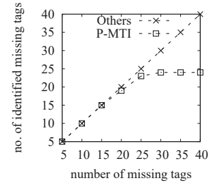
Fig. 4: Number of identified missing tags by P-MTI, and other protocols including DBF, THP, SFMTI and Protocol 3.
