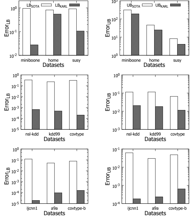
Fig. 13: Error_{LB} and Error_{UB} for Type-I, II and III queries
