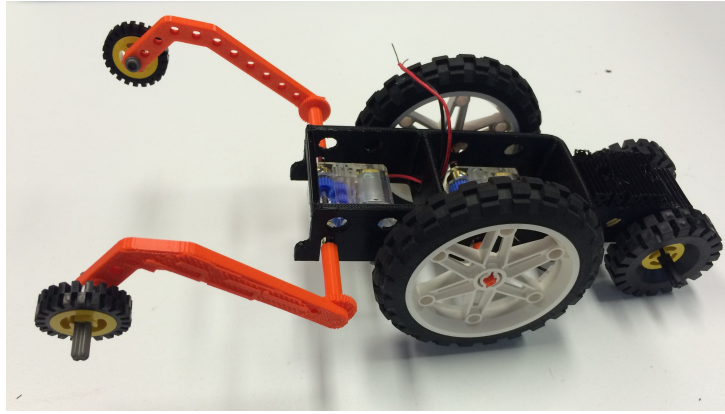
Figure 8: An example of the hurdle robot designed and built by the students
