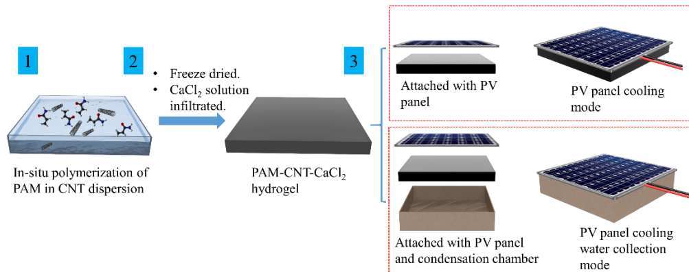
Figure 1. Schematic of PAM-CNT- \text{CaCl}_2 cooling layer synthesis process (step 1 and 2) and two PV panel working modes (step 3).
