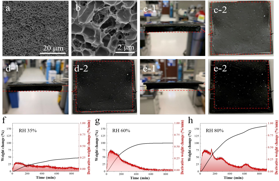
Figure 2. (a) SEM image and (b) magnified SEM image of freeze-dried PAM-CNT hydrogel. Digital photo of PAM-CNT-CaCl 2 hydrogel attached on the backside of a commercialized PV panel (c) before water vapor desorption; after water vapor desorption for (d) 1.5 h and (e) 3 h under simulated sunlight strength of 1 kW/m 2 . The hydrogel was cut into a squared shape by knife. The dash lines indicate the thickness change of the hydrogel during test, and the dash square indicates the dimension change of the hydrogel during the test. (f)-(h) Water vapor sorption properties of PAM-CNT-CaCl 2 hydrogel under different RH conditions at 25 °C.
