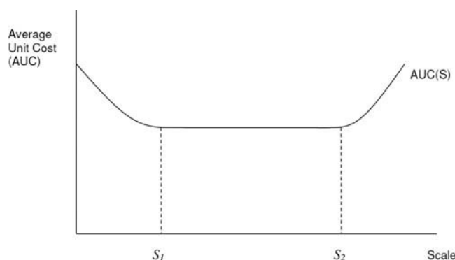
Figure 2. McDonnell/Stigler relationship between unit cost and scale (McConnell, 1945; Stigler, 1958).
