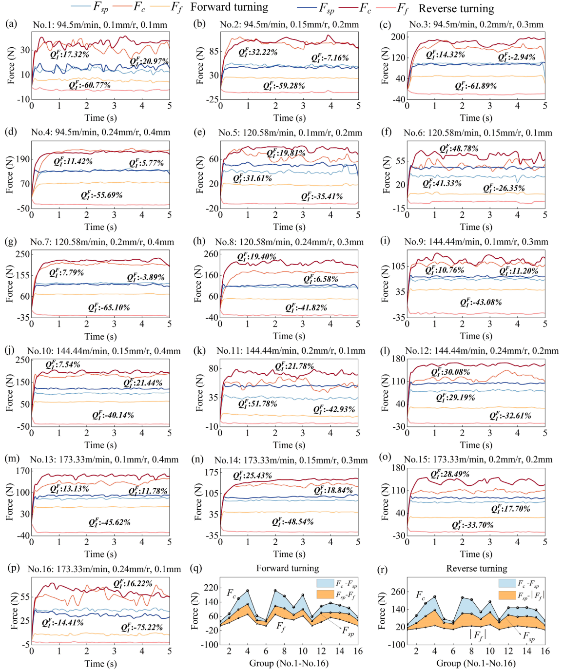
Fig. 11. Experimental triaxial forces for forward and reverse turning for different cutting parameters. The effect of cutting speed are shown in (a)–(d) first level, (e)–(h) second level, (i)–(l) third level and (m)–(p) fourth level. Factor Q_i^F is calculated as (F_{Reverse} - F_{Forward}) / F_{Forward} . The tangential and radial forces of reverse turning are generally higher than those of forward turning, and the axial forces of reverse turning are smaller than those of forward turning and in the opposite direction. The tangential force is significantly greater than the radial and axial forces in the triaxial force of (q) forward turning and (r) reverse turning for each group.
