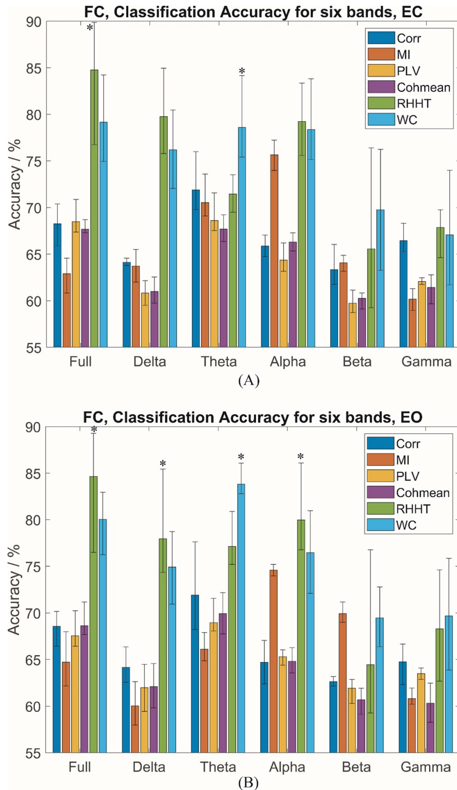
Figure 9. Comparison of the RHHT and previous brain connectivity methods. * Mann–Whitney test, p < 0.001 , it means significant outperformance in a band.
