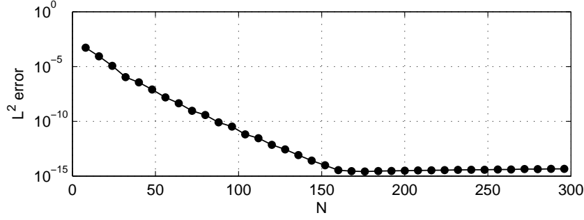
FIGURE 1. Spectral accuracy in space for the ETD1 scheme (2.10).
