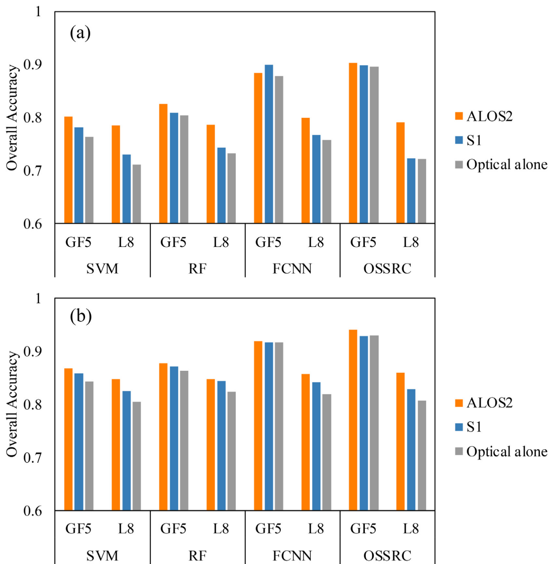
Fig. 6. Mean overall accuracy using different data groups. (a): Case 1, (b): Case 2.
