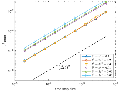
FIG. 1. Temporal convergence rates in Example 4.1.
