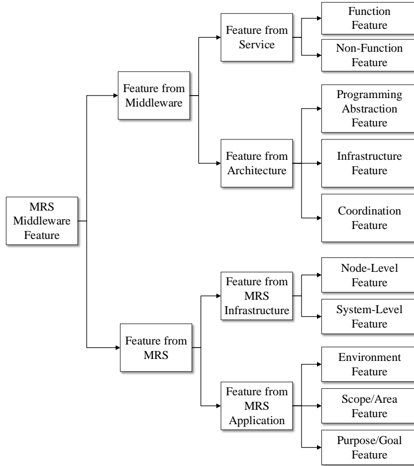
Fig. 5: Overview of feature tree of MRS middleware
