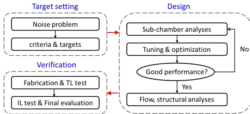
Fig. 13—Flowchart of the cascade muffler design.
