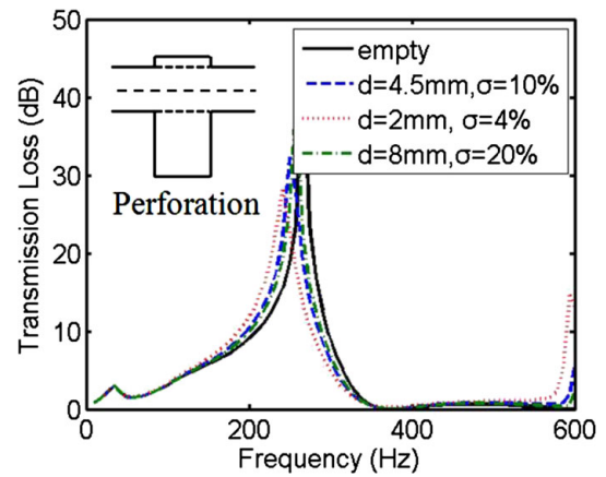
Fig. 5—Effect of varying parameters of the perforated duct, chamber width, w = 0.3 m.
