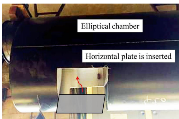
Fig. 8—Modification on the existing muffler: the second sub-chamber is reshaped by inserting a horizontal plate (refer to Fig. 6).
