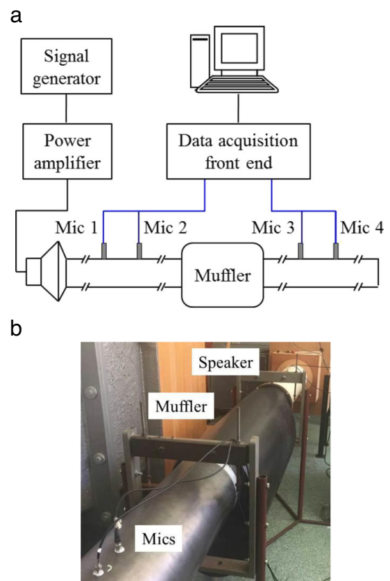
Fig. 9—(a) Test-rigs based on four-microphone method to measure the muffler TL; (b) The actual muffler configuration.
