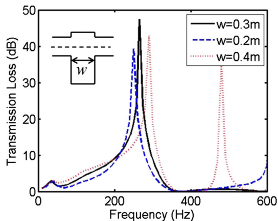
Fig. 4—Effect of varying width, w , of an empty sub-chamber.
