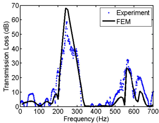
Fig. 10—Comparison between measured and simulated TLs for the original muffler in Fig. 1.
