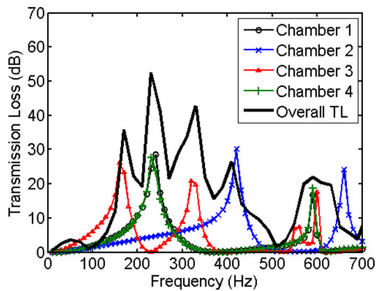
Fig. 7—Simulated sub-chamber TLs and overall TL of the retrofitted muffler.
