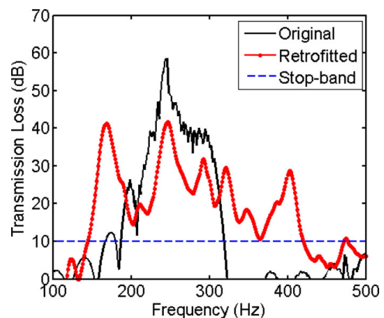
Fig. 12—The measured TLs of the original and retrofitted muffler from 100 to 500 Hz.
