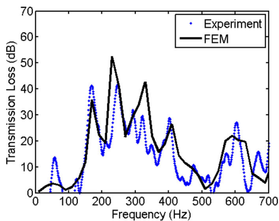
Fig. 11—Comparison between measured and simulated TLs for the retrofitted muffler in Fig. 6.
