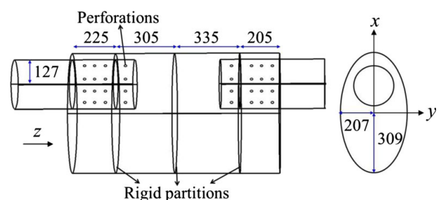
Fig. 1—Geometry and dimensions of the original muffler, in mm.
