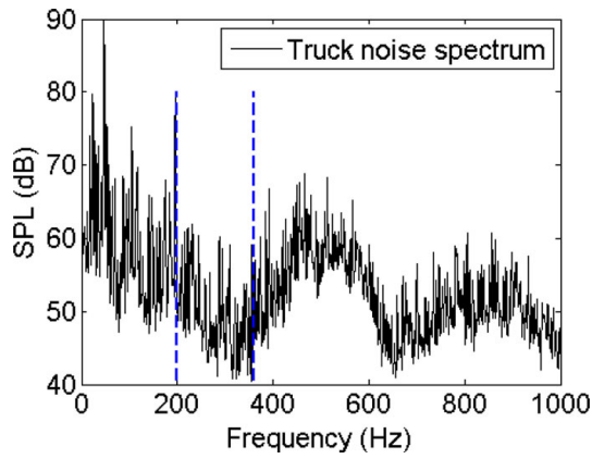
Fig. 3—Noise spectrum measured 10 m away from the muffler, with the truck in high idle condition.
