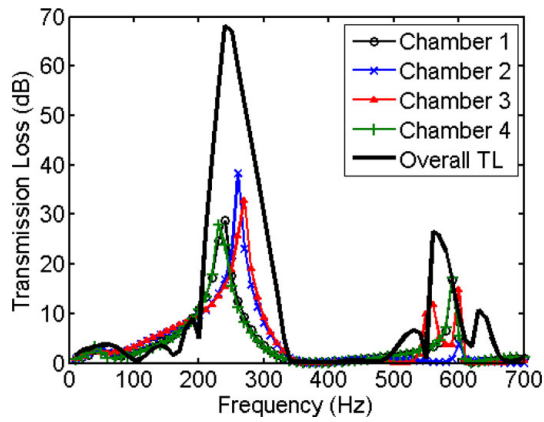
Fig. 2—Predicted TL characteristics of the sub-chambers and the overall muffler TL.
