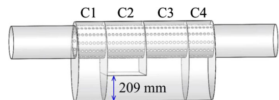
Fig. 6—Configuration of the retrofitted muffler design. The outer dimension of the elliptical chamber and the diameter of the inlet/outlet duct remain unchanged, the same as in Fig. 1.
