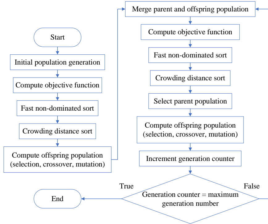
Fig. 4. Flow-chart of the main procedure of the NSGA-II.
