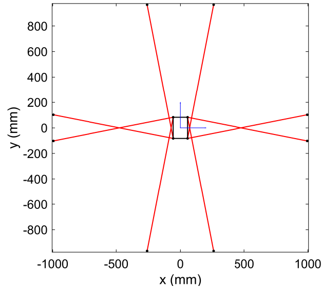
Fig. 6. The obtained differentially driven CPR from multi-objective optimal design.
