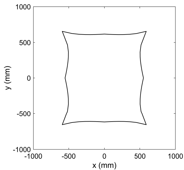
Fig. 10. The boundary of the TOWCW of the obtained fully actuated CPR.
