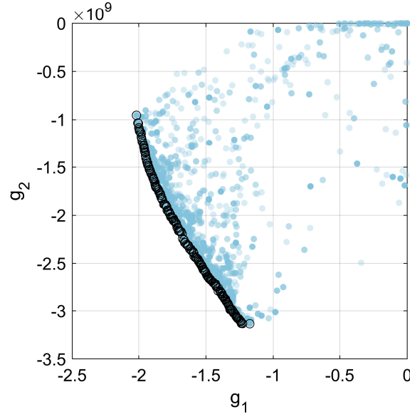
Fig. 5. The optimization process using the NSGA-II for the differentially driven CPR.
