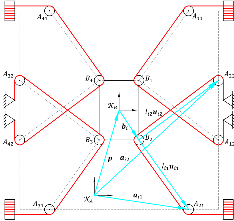
Fig. 3. Schematic of the planar differentially driven CPR.
