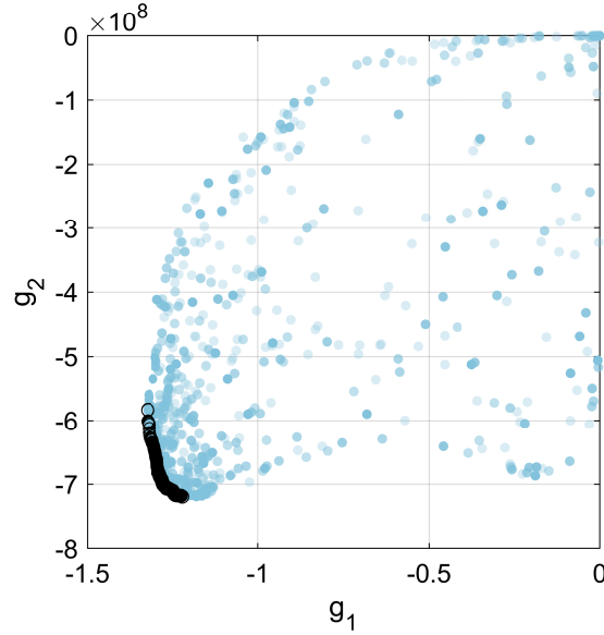
Fig. 8. The optimization process using the NSGA-II for the fully actuated CPR.
