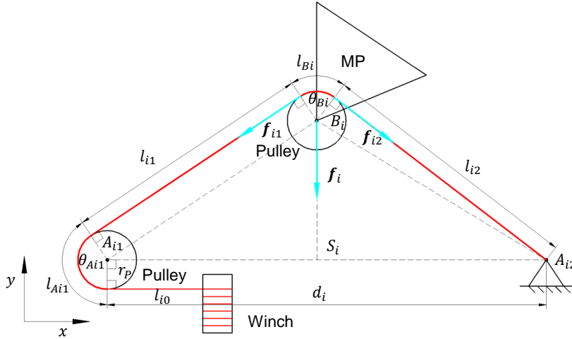
Fig. 1. Schematic of the i -th cable and pulley differential on the CPR.
