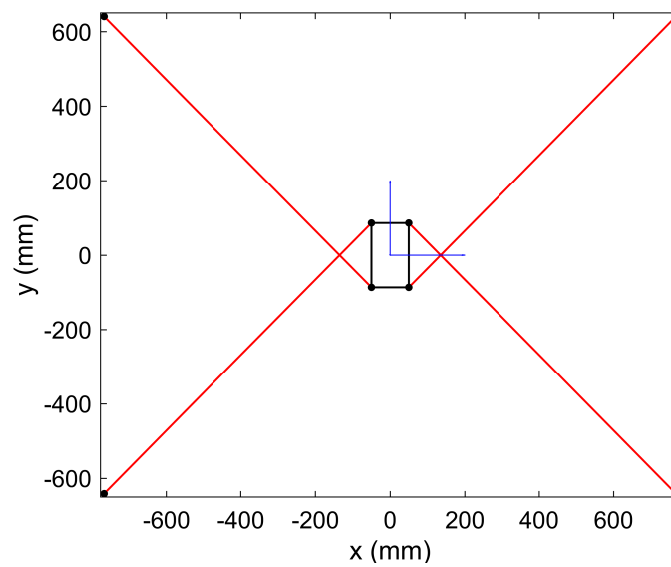
Fig. 9. The obtained fully actuated CPR from multi-objective optimal design.
