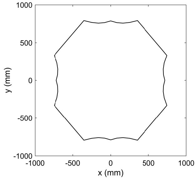
Fig. 7. The boundary of the TOWCW of the obtained differentially driven CPR.
