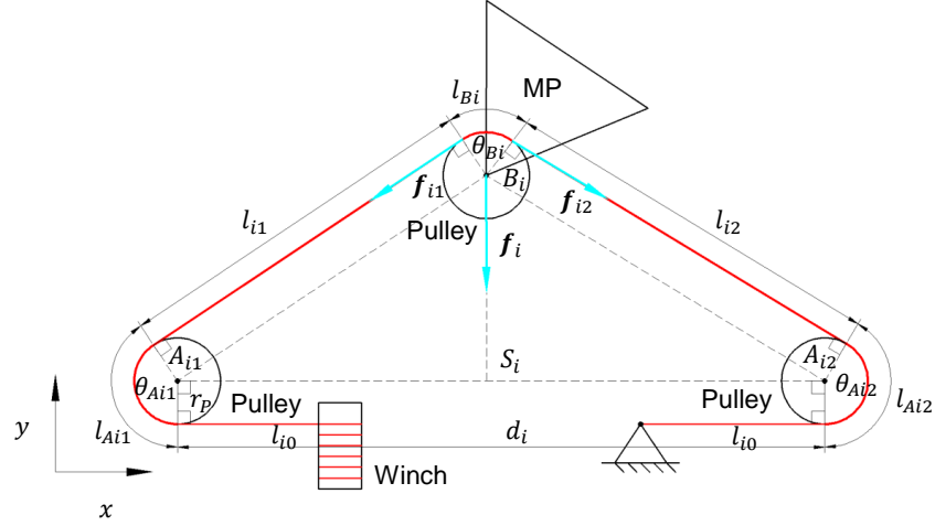
Fig. 2. Schematic of the i -th cable and pulley differential with extra pulley on the CPR.
