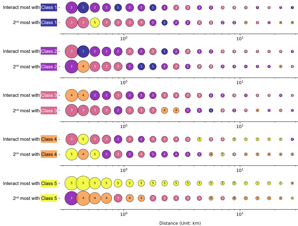
Figure 7: The classes that interact most and second most with each of the five classes at a given distance. Size of dot is proportional to the normalized communication frequency between the corresponding classes.
