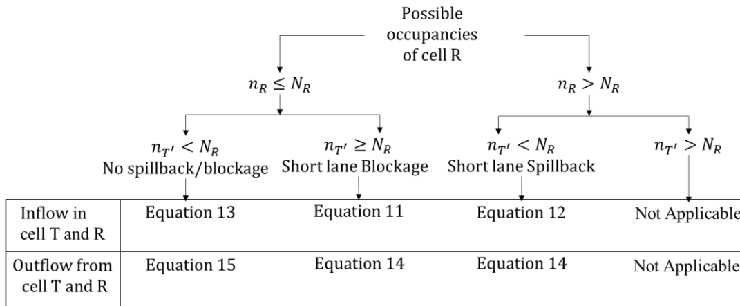
Figure 6: Combination of cell occupancies in the presence of the short turning lane
