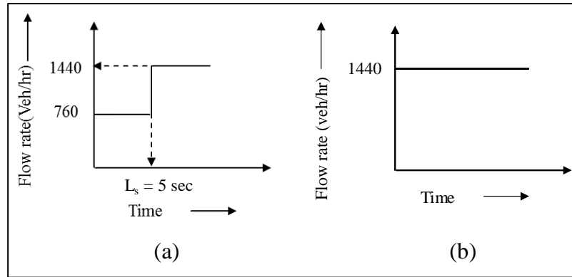
Figure 19: Flow rate profile for the CTM simulation a) ACTM; b) traditional CTM
