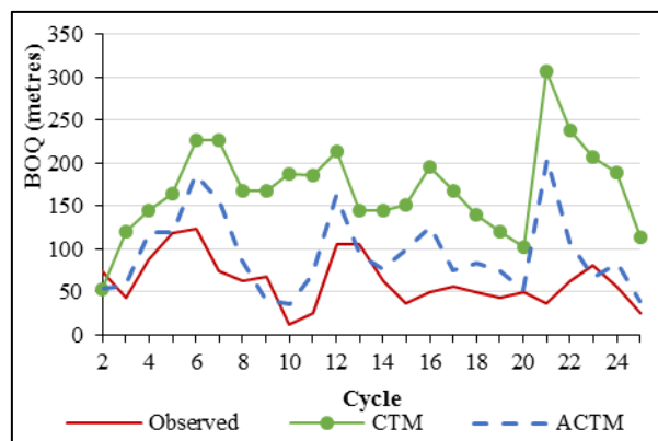
Figure 21: BOQ comparison for Site 2
