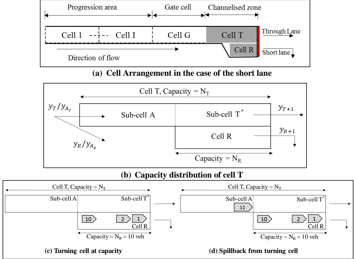
Figure 5: Proposed set up for the CTM in the case of the short turning lane
