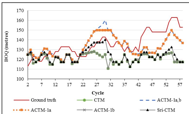
Figure 10: BOQ comparison considering a modification in the queue-discharge process in the ACTM (refer to Section 3.1) for Case-1: Under-saturated traffic condition
