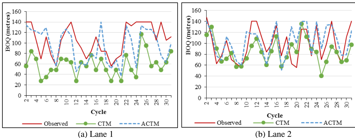
Figure 20: BOQ comparison for Site 1
