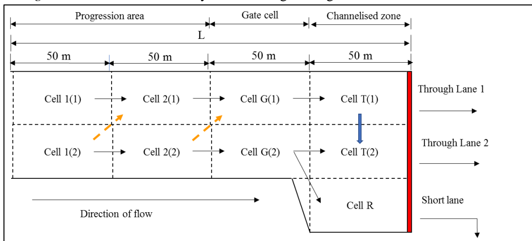
Figure 15: Experiment details for lane utilisation balancing
