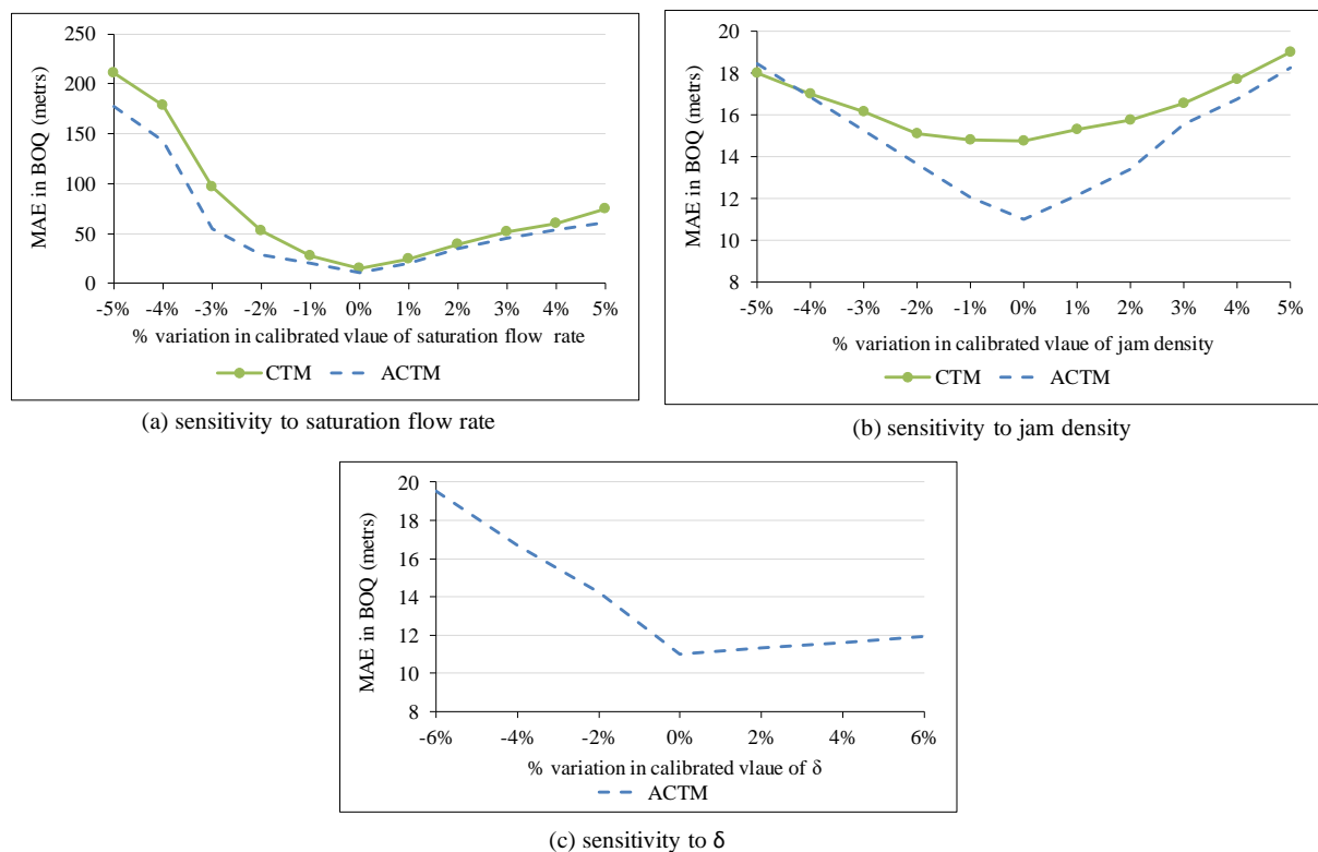
Figure 17: Sensitivity analysis for CTM and ACTM
