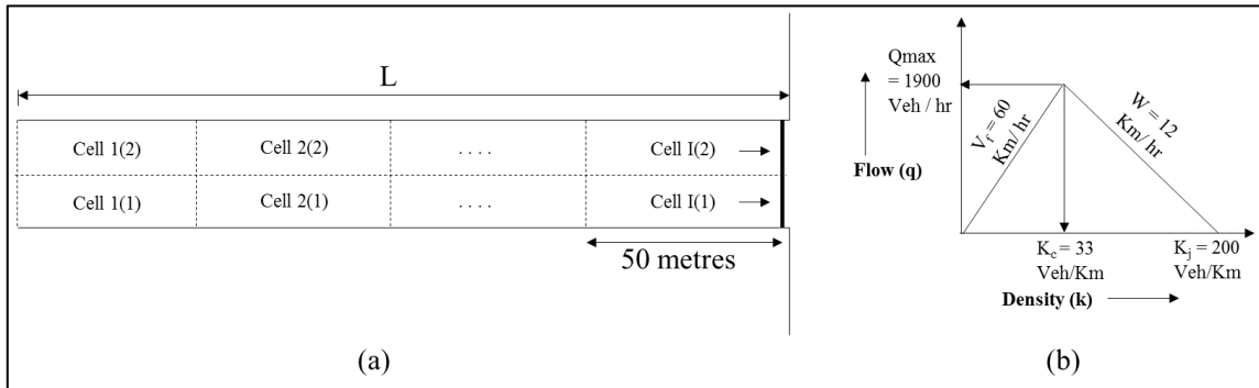
Figure 9: Experiment details for the queue discharge process modification in ACTM
