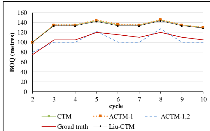
(b) Case – 2: short lane length less than cell length
