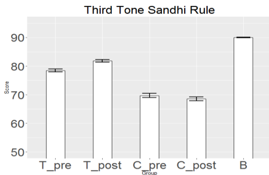
Figure4. Mean scores of tone productions in T3+T3
