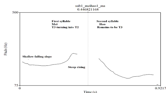
Figure2. F0 contour of “/mәi3/ /xau3/”with tone sandhi
