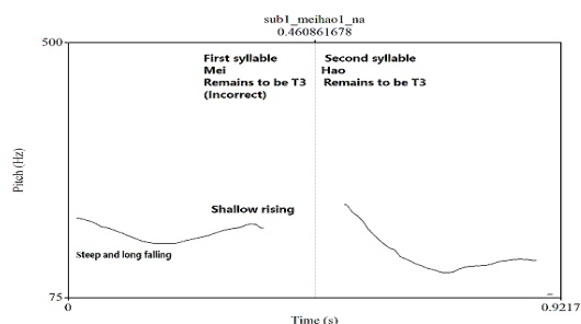
Figure1. F0 contour of “/mәi3/ /xau3/”without tone sandhi
