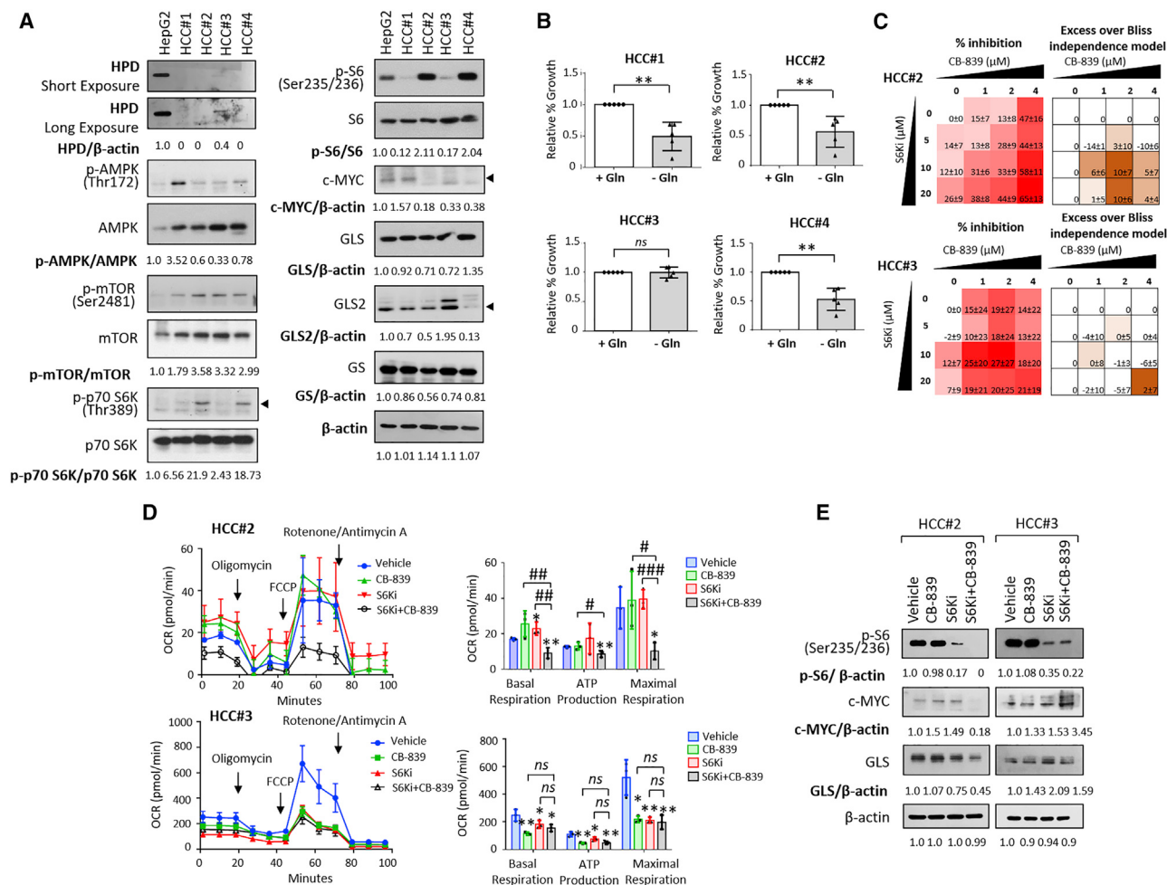
Figure 6. Combination treatment of p70S6 kinase and GLS inhibition exerts synergistic growth inhibition effect in human HCC organoids with HPD downregulation
