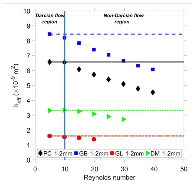
FIGURE 14 | Effective permeability ( k_{\text{eff}} ) as a function of Reynolds number. PC, pine chips; GB, gum bark; GL, gum leaf; DM, decomposing matter.
