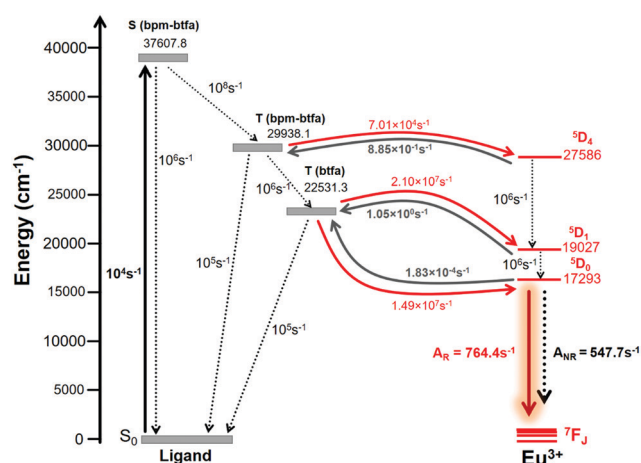
Fig. 6 Schematic energy-level diagram, ET processes, and transfer rates considered for 1 . The rates shown are typical experimental values for the non-radiative rates in coordination compounds. 28
