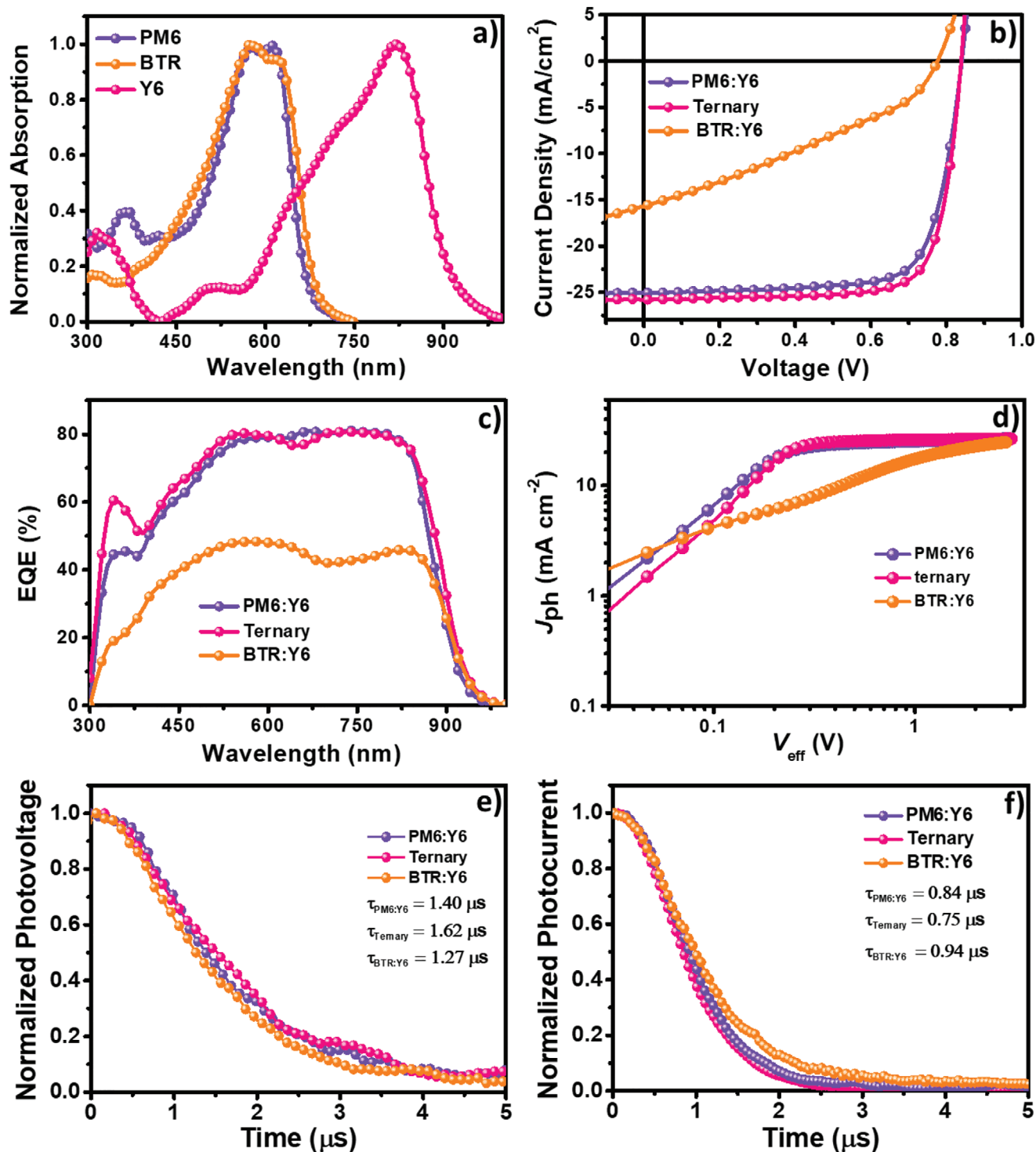
Figure 1. a) Normalized UV-vis absorption of PM6, BTR, and Y6 pristine films. b) Current density–voltage ( J - V ) curves. c) EQE, d) J_{\text{ph}} versus V_{\text{eff}} , e) TPV, and f) TPC of OSC devices based on PM6:Y6, PM6:BTR:Y6 (0.95:0.05:1.2), and BTR:Y6 blends.
