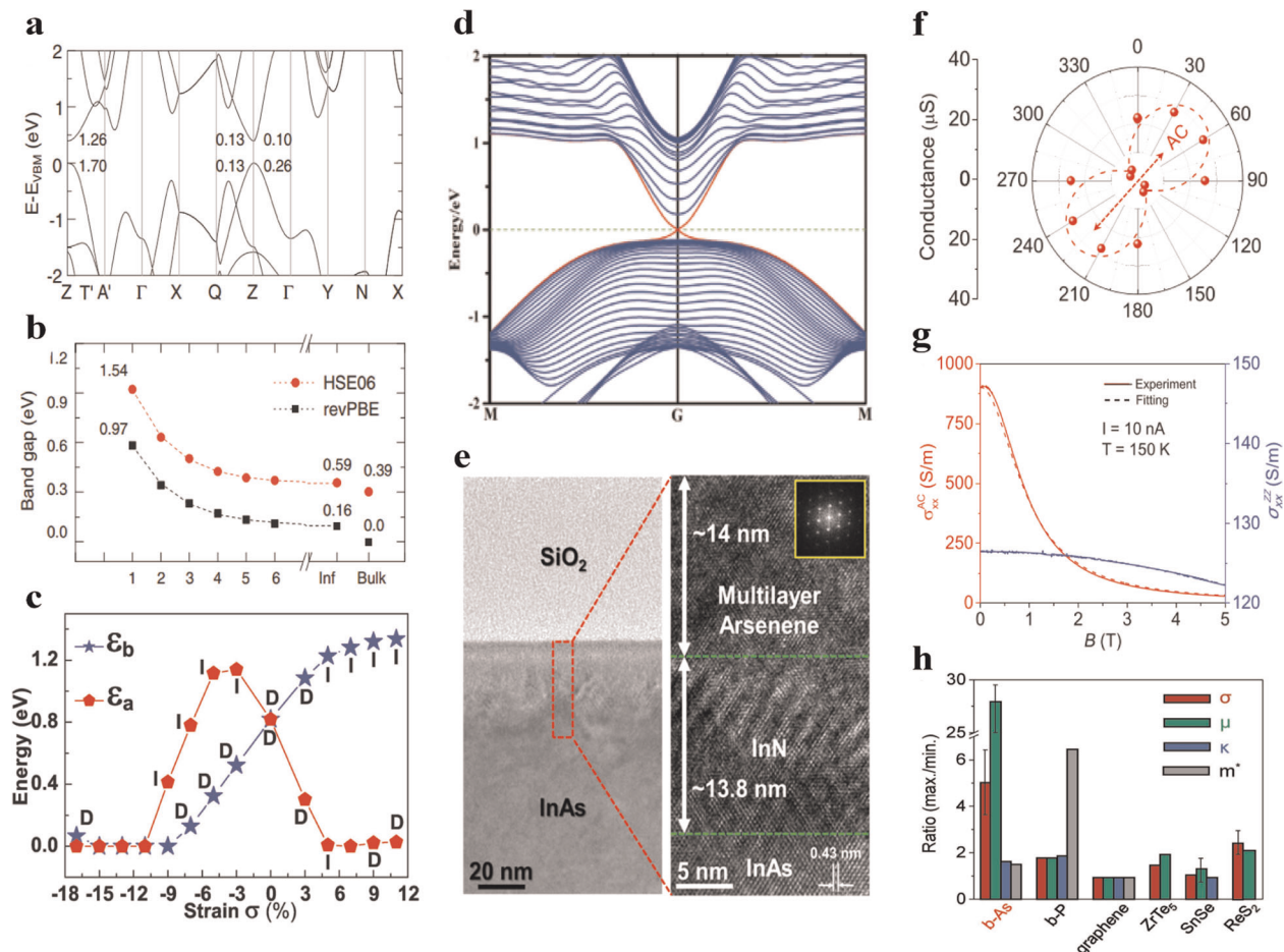
Fig. 5 | Electrical transport properties of arsenic ultrathin 2D layer. a Calculation of the band structure for orthorhombic arsenene, showing its direct bandgap. b Layer dependence of the energy bandgap of \alpha -arsenene. c Variation of the bandgap of \alpha -arsenene, including direct (marked by letter D)/indirect (marked by letter I) energy band, as a function of the applied strain along zigzag ( \epsilon_a ) and armchair ( \epsilon_b ) directions. d The tuning tendency of the electronic structure for \beta -arsenene nanoribbon with zigzag edge, constructing with a 11.7% tensile strain, from which the helical edge states could be prospected at G point. e Cross-sectional transmission electron microscope images of the multilayer arsenene synthesized by plasma-assisted process. f Angle-dependent appearance on electrical conductance of \alpha -arsenene, exhibiting the preferred transportation along armchair (AC) direction. g Magnetic-field-dependent conversion of longitudinal conductivity \sigma_{xx} along armchair (AC) and zigzag (ZZ) directions. h Comparison of the in-plane anisotropic electrical transport properties of \alpha -arsenene and some other 2D materials. Images of a and b adapted with permission from ref. 21 copyright (2015) The Japan Society of Applied Physics. Image of c republished with permission of Royal Society of Chemistry, from ref. 96 ; permission conveyed through Copyright Clearance Center, Inc. Image of d republished with permission of Royal Society of Chemistry, from ref. 100 ; permission conveyed through Copyright Clearance Center, Inc. Image of e adapted with permission from ref. 51 copyright 2016, American Chemical Society. Images of f–h used with permission from John Wiley and Sons 101 .
