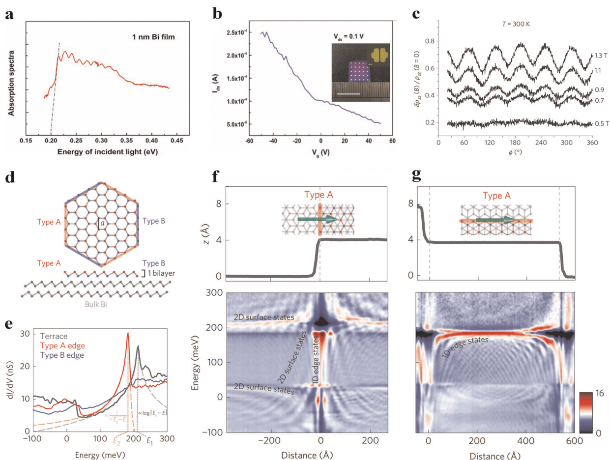
Fig. 7 Electrical transport properties of bismuth ultrathin 2D layer. a Absorption spectrum for 1-nm bismuthene sample, showing tiny bandgap of ~0.2 eV. b Typical p-type transferring characteristic examined from one 10-nm-Bi-based FET. The inset shows 25 FETs evenly distributed across the centimeter plane of Bi ultrathin film. c Magnetic resistance performance of bismuth monocrystal with significant angular dependence that are investigated under different magnitudes of external magnetic field. d Schematics of two different edge types in bismuthene monolayer, showing by planar view and side view. e Point spectroscopy spectra of the dI/dV value as a function of the energies. Red, blue, and gray line are referred to the measurements along type A edge, along type B edge, and on the uniform surface, respectively. f, g Topographic line-cut feature and spectroscopy with energy line-scanning across and along the type A edge, respectively, which clearly exhibited the 1D edge state. Images of a and b used with permission from John Wiley and Sons 43 . Image of c used with permission from Springer Nature 131 . Images of d–g used with permission from Springer Nature 137 .
