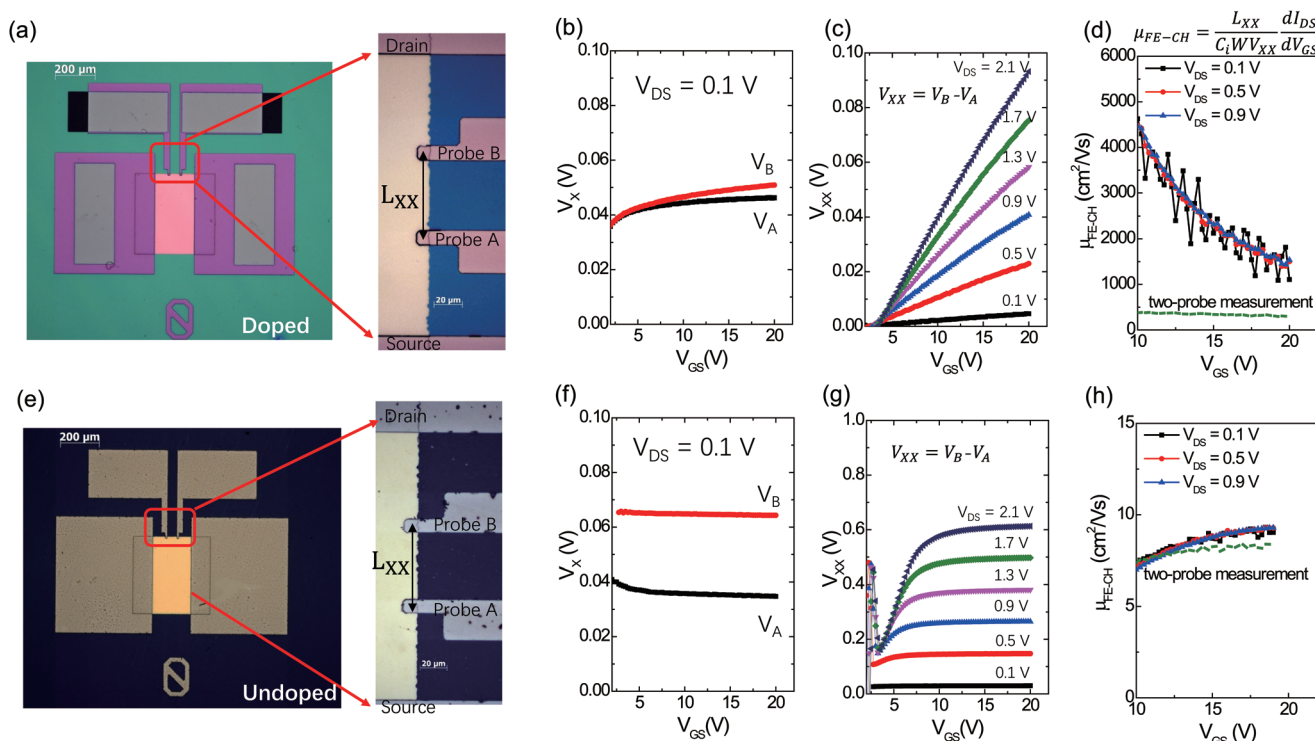
Figure 3. Gated four-probe (GFP) measurements. a) Optical image of one IGZO-H TFT and the region near the probes is enlarged on the right. b) Potential of probe A and B in IGZO-H TFT with V_{DS} = 0.1 V. c) Potential drop V_{XX} = V_B - V_A as a function of V_{GS} with various V_{DS} . d) The extracted channel field-effect mobility of IGZO-H TFT with various V_{DS} by GFP measurements (dots) or transfer curves of TFTs (dashed lines). The corresponding measurements of IGZO TFT are shown in (e–h).
