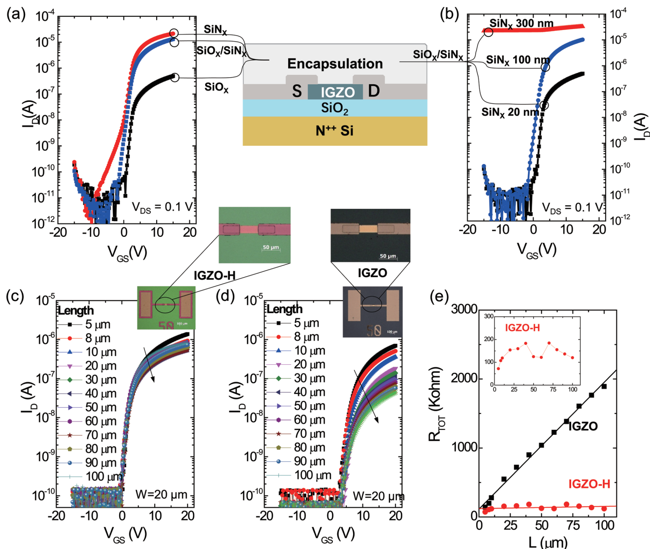
Figure 2. Effect of encapsulation layers and channel length scaling. a) Linear transfer curves with encapsulation layer of \text{SiO}_x (350 nm, black), \text{SiN}_x (100 nm, red), or \text{SiO}_x/\text{SiN}_x (350/100 nm, blue). b) Linear transfer curves with encapsulation layer of \text{SiO}_x/\text{SiN}_x with varying the thickness of \text{SiN}_x : 20 nm (black), 100 nm (blue), or 300 nm (red). All the devices were annealed at 350 °C for 1 h after the final deposition. Transfer characteristics ( V_{DS} = 0.1 V) of IGZO-H c) and IGZO d) TFTs with channel length L varying from 5 to 100 \mu\text{m} ( W = 20 \mu\text{m} ) with optical images. The zoomed-in images show the channel area with the semiconductor islands is narrower than the electrodes, avoiding the fringe current. e) Total resistance R_{TOT} against L for IGZO TFTs (black) and IGZO-H TFTs (red), with the latter enlarged as inset. The dots are measured data and the lines are linear fittings.
