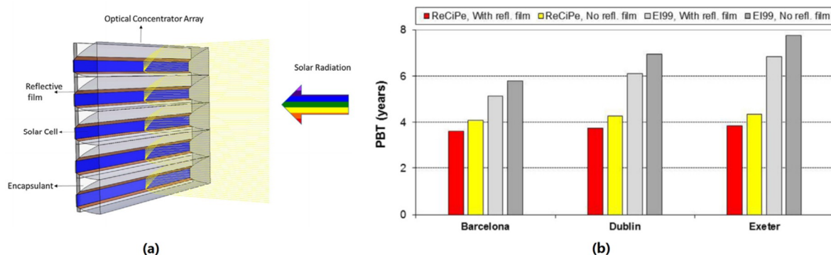
Figure 8. The environmental assessment of (a) a building-integrated concentrating photovoltaic (BICPV) according to (b) the multiple life-cycle indicators in Reference [75].
