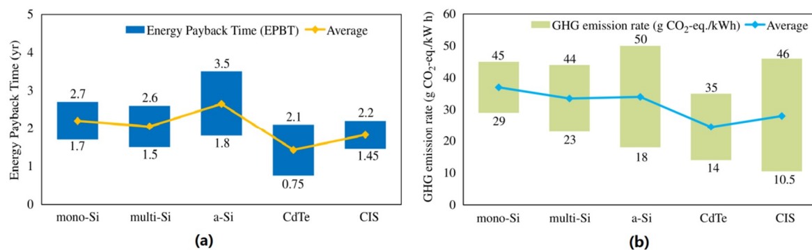
Figure 9. The review results of (a) energy payback time (EPBT) and (b) the greenhouse gas emission (GHGE) rate for various PV modules [89].
