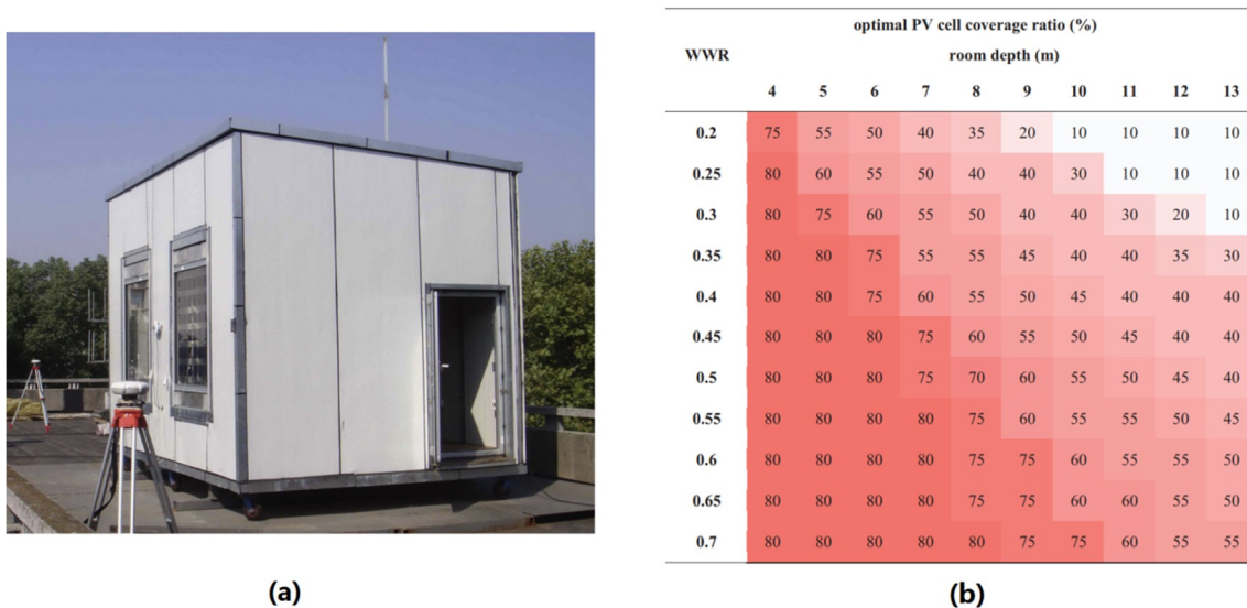
Figure 5. (a) A ventilated semi-transparent photovoltaic (PV) façade and its (b) optimal PV cell coverage ratio under various window-to-wall ratios and room depths [55].
