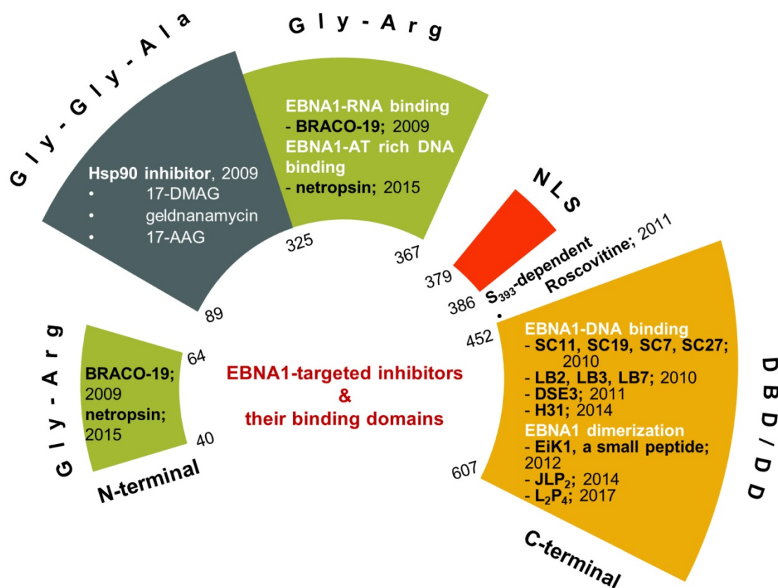
Figure 3. Recent developments of EBNA1 inhibitors. The inhibitors are shown in their respective EBNA1 domains.
