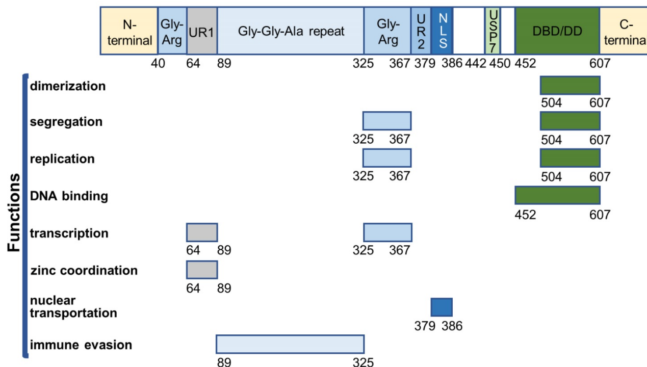
Figure 2. Overview of EBNA1 functional domains.
