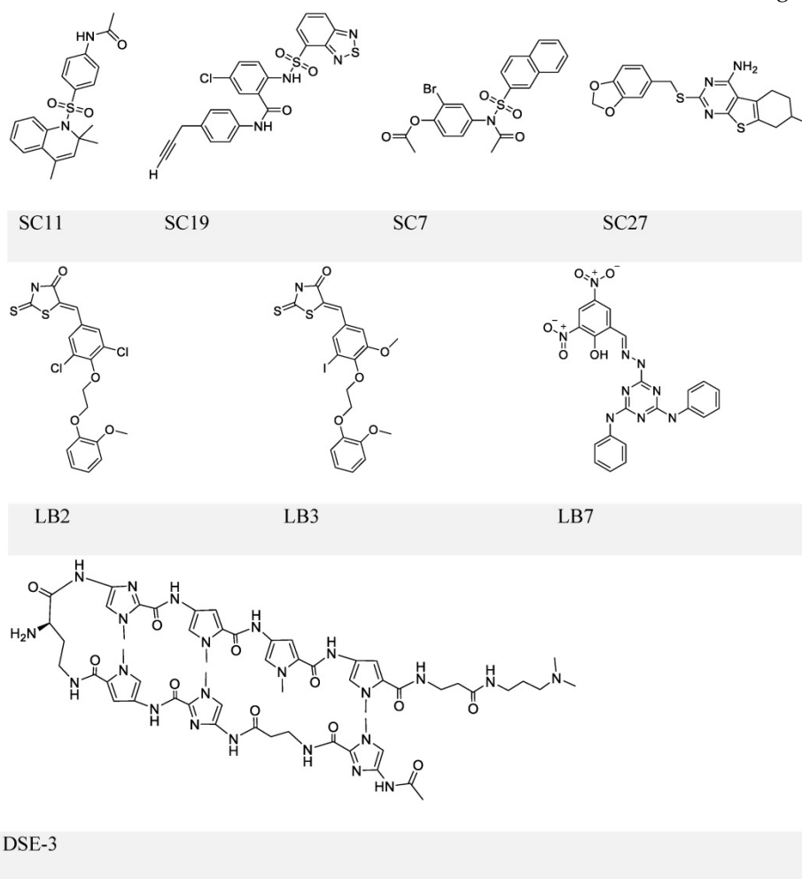
Figure 5. Chemical structures of EBNA1-DNA binding inhibitors. Inhibitors in the upper and middle panel are identified via screening approaches that could block EBNA1-DNA binding. The inhibitor in the lower panel is a known DNA ligand that competitively binds the EBNA1-bound site on DNA.
