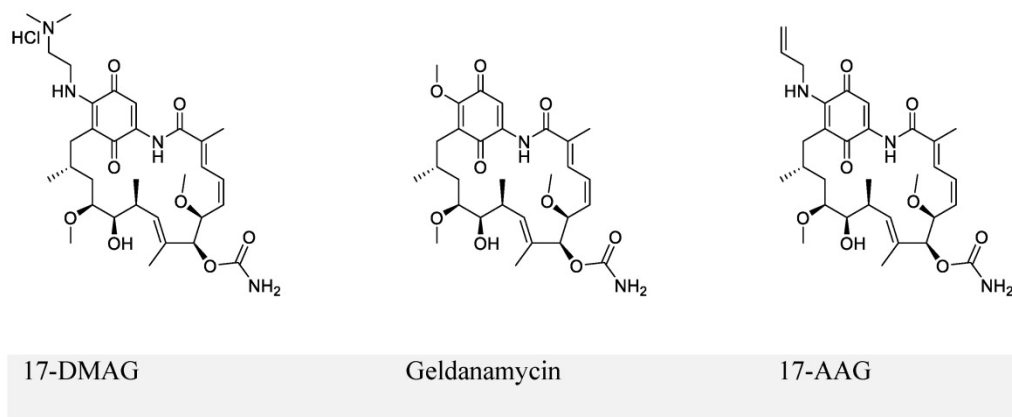
Figure 4. Chemical structures of Hsp90 inhibitors.
