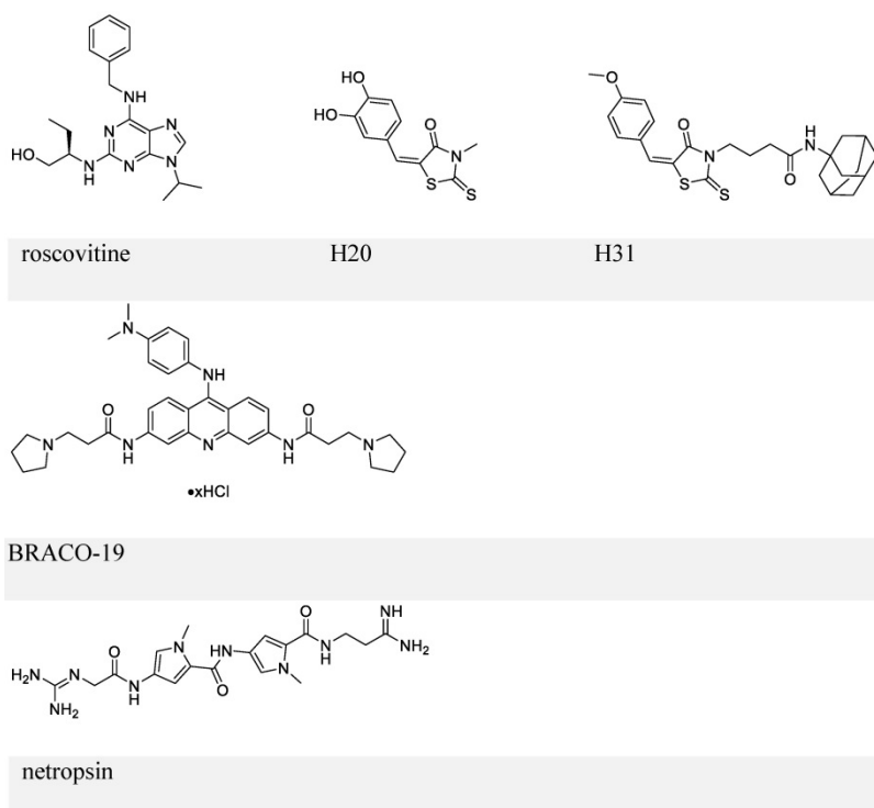
Figure 6. Chemical structures of inhibitors that block EBNA1-oriP transactivation and EBNA1 Gly-Args-dependent functions.
