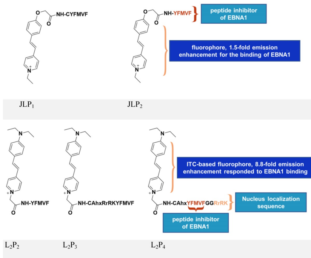
Figure 7. Chemical structures of inhibitors based on peptides from EBNA1 DBD/DD. Adapted with permission from [118, 119], copyright 2014 The Royal Society of Chemistry and 2017 Springer Nature.
