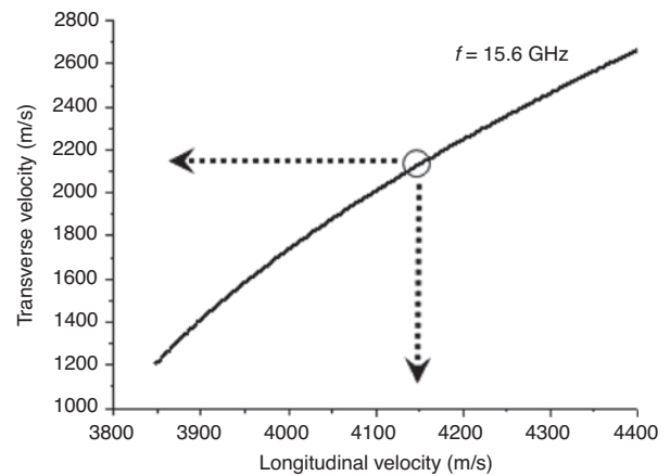
Figure 20: Black curve corresponding to the different couples of v_l and v_t which give the first breathing mode frequency equal to 15.6 GHz obtained in 91 nm diameter single copper nanowires [109]. The black arrow pointed out the standard velocities in polycrystalline copper around 4150 \text{m}\cdot\text{s}^{-1} and 2150 \text{m}\cdot\text{s}^{-1} , respectively, for longitudinal and transverse sound velocity.
