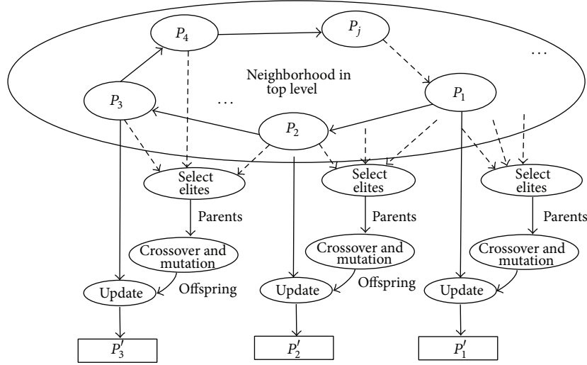
FIGURE 2: The information exchange mechanism based on crossover operator.
