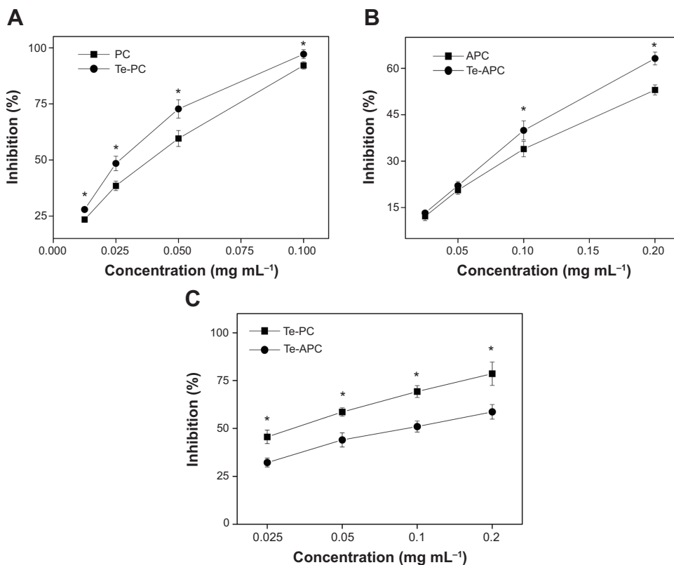
Figure 5 (A) Antioxidant activities of Te-PC and (B) Te-APC as determined by ABTS assay and (C) hemolysis assay.
