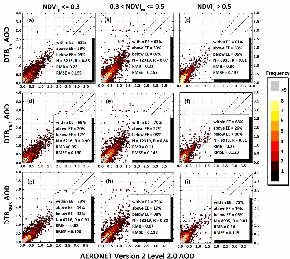
Figure 7. Validation of an equal number of the DTB C6 (a–c), DTB C6.1 (d–f) and DTB SMS (g–i) AOD retrievals for the same geolocations (time and place) against the same AERONET L2 V2 AOD measurements for 68 global sites located over NDVI P , NDVI M , and NDVI D surfaces. Where dashed lines represent the EE envelope and the solid line represents the 1:1 line.
