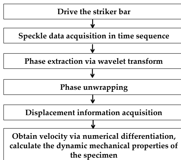
Figure 4. Signal processing flowchart.
