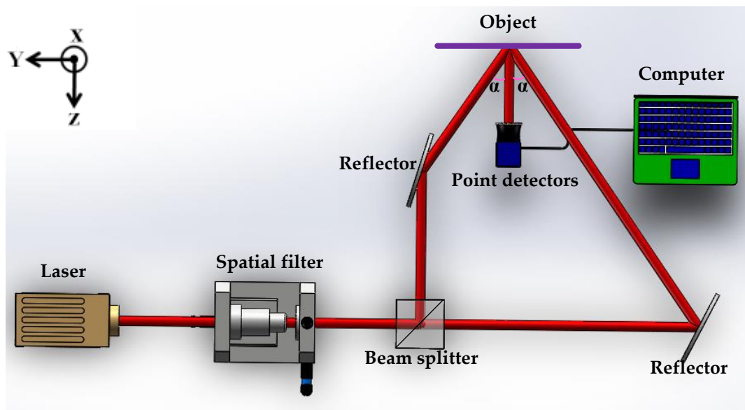
Figure 2. The optical path of in-plane displacement measurement.
