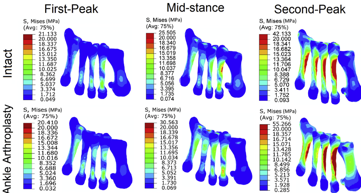
Figure 7 Comparison of von Mises stress distribution in metatarsals between models of the intact foot and total ankle arthroplasty foot at the first-peak, mid-stance and second-peak instants.
