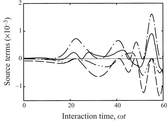
FIGURE 16. Time variation of source terms due to vortex centroid dynamics during partial coalescence. C/y_{20} = 1.5 . —, \sum \Gamma y_{c2}(\partial^3 y'_{c1}/\partial t^3) ; — —, \sum 3\Gamma(\partial y_{c2}/\partial t)\partial^2 y'_{c1}/\partial t^2 ; — · —, \sum 3\Gamma(\partial y'_{c1}/\partial t)\partial^2 y_{c2}/\partial t^2 ; — — —, \sum \Gamma y'_{c1}(\partial^3 y_{c2}/\partial t^3) .
