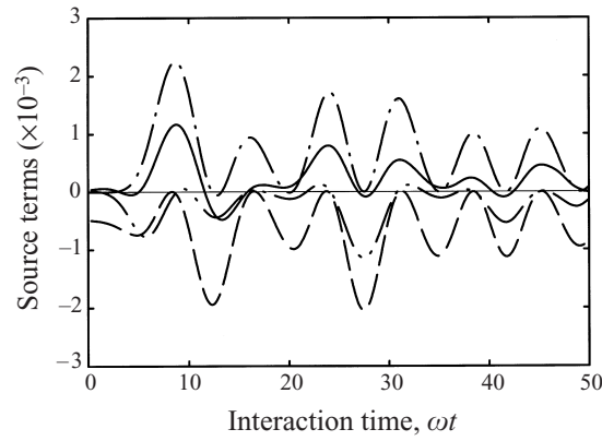
FIGURE 21. Time variations of source terms due to vortex centroid dynamics during coalescence. C/y_{2o} = 1 . —, \sum \Gamma y_{c2}(\partial^3 y'_{c1}/\partial t^3) ; ---, \sum 3\Gamma(\partial y_{c2}/\partial t)\partial^2 y'_{c1}/\partial t^2 ; — · —, \sum 3\Gamma(\partial y'_{c1}/\partial t)\partial^2 y_{c2}/\partial t^2 ; · · · ·, \sum \Gamma y'_{c1}(\partial^3 y_{c2}/\partial t^3) .
