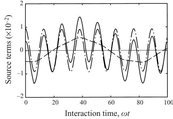
FIGURE 23. Source terms for two-dimensional vortex leapfrogging case (cf. figure 10 of Tang & Ko 1997). —, \ddot{S} ; — —, \ddot{S}_2 = \Gamma(\partial^3/\partial t^3)(y_{c2}y'_{c1}) ; — · —, \ddot{S}_1 = \Gamma y_{c2}(\partial^3/\partial t^3)(y_{ic1} - y_{c1}) .
