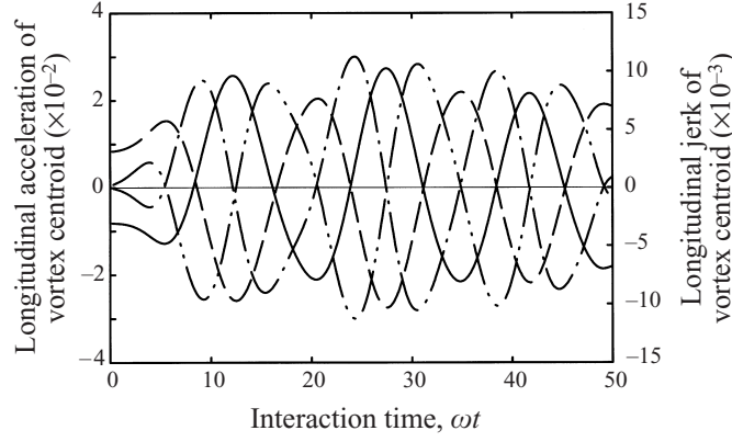
FIGURE 18. Time variation of longitudinal accelerations and jerks of vortex centroids during coalescence. C/y_{2o} = 1 . —, Acceleration of initially leading vortex centroid; — — —, jerk of initially leading vortex centroid; — · —, acceleration of initially trailing vortex centroid; · · · —, jerk of initially trailing vortex centroid.
