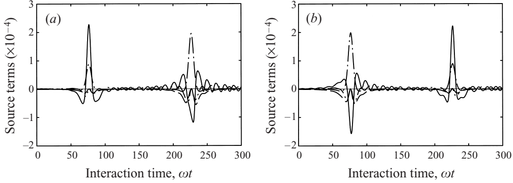
FIGURE 6. Decomposition of source term \ddot{S}_2 . (a) Initially leading vortex pair; (b) initially trailing vortex pair. —, \Gamma y_{c2} \partial^3 y'_{c1} / \partial t^3 ; — —, 3\Gamma (\partial y_{c2} / \partial t) \partial^2 y'_{c1} / \partial t^2 ; — · —, 3\Gamma (\partial^2 y_{c2} / \partial t^2) \partial y'_{c1} / \partial t ; — — —, \Gamma y'_{c1} (\partial^3 y_{c2} / \partial t^3) .
