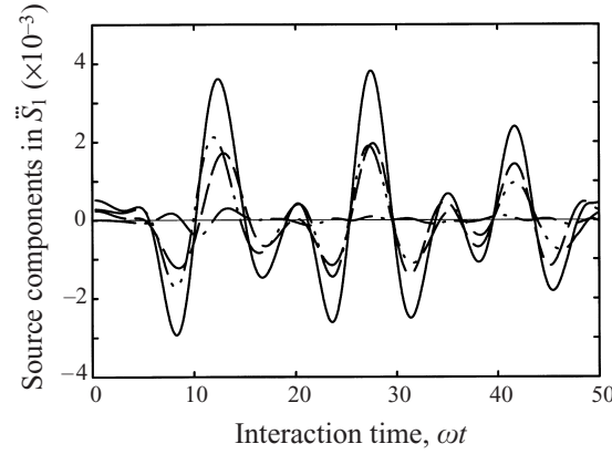
FIGURE 20. Relative importance of different components in \sum \ddot{S}_1 during coalescence. C/y_{2o} = 1 . —, \sum \Gamma y_{c2}(\partial^3/\partial t^3)(y_{ic1} - y_{c1}) ; ---, R ; — · —, \Gamma y_{c2}(\partial^3/\partial t^3)(y_{ic1} - y_{c1}) of initially leading vortex pair; · · · ·, \Gamma y_{c2}(\partial^3/\partial t^3)(y_{ic1} - y_{c1}) of initially trailing vortex pair.
