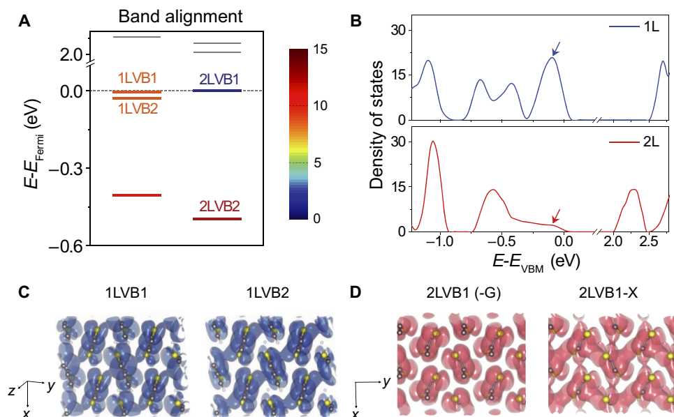
Fig. 4. Calculated electronic and contact properties. (A) Band alignment of Au/1L and Au/2L metal-semiconductor junction. Four valence states responsible for the hole transport are marked (the band structure is shown in fig. S8). The color of these states indicates different DOSs as shown by the color bar. (B) Total DOS for 1L (blue solid line) and 2L C_8 -BTBT (red solid line). Blue and red arrows mark the highest-energy valence bands for 1L and 2L, respectively. (C) Spatial distribution of the molecular orbitals at G point for 1LVB1 and 1LVB2. (D) Spatial distribution of the molecular orbitals at G and X point (0.5, 0, 0) for 2LVB1 using an isosurface of 0.0005 \text{ e bohr}^{-3} .
