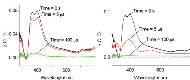
Fig. 7 Left: Time resolved absorption difference spectra of Pd-B-1 ( 5 \times 10^{-5} \text{ mol dm}^{-3} ) in degassed CH 3 CN monitored at 0 s, 5 \mu\text{s} and 100 \mu\text{s} ; Right: time resolved absorption difference spectra of Pd-B-1 ( 5 \times 10^{-5} \text{ mol dm}^{-3} ) and TMEDA ( 0.69 \text{ mol dm}^{-3} ) in CH 3 CN monitored at 0 s, 5 \mu\text{s} and 100 \mu\text{s} .
