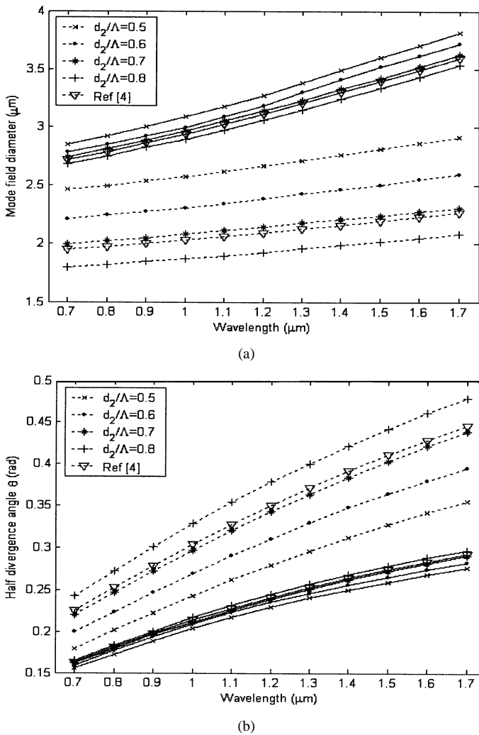
Fig. 5. (a) The mode field width ( w_x : the dotted lines; w_y : the solid lines) of the y -polarized mode as function of wavelength for various d_2/\Lambda . (b) The half divergence angles ( \theta_x : the dotted lines; \theta_y : the solid lines) of the y -polarized mode as a function of wavelength for various d_2/\Lambda .
